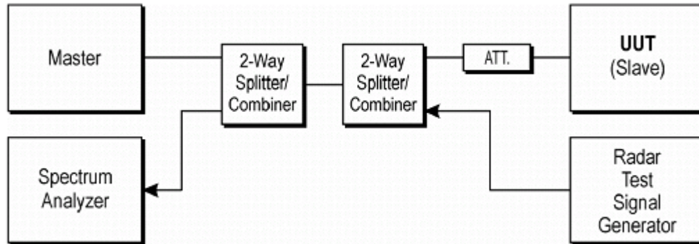
Figure 7-1. Test Setup
