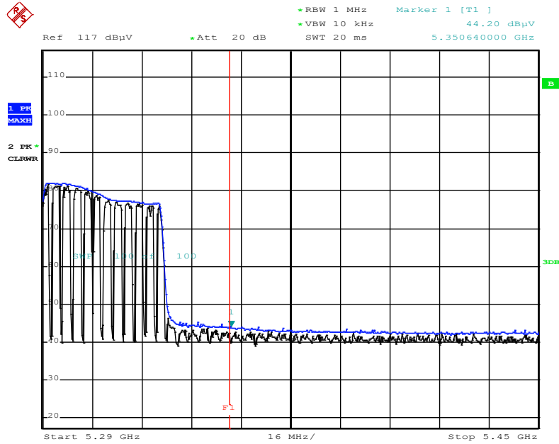
Average Reading (802.11ac_VHT80, Ch.58)
