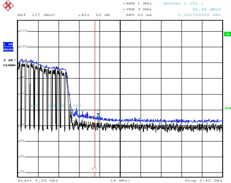
Peak Reading (802.11ac_VHT80, Ch.58)
