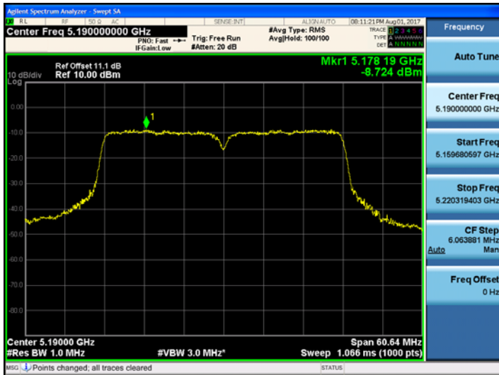
802.11n_HT40 UNII 1 BAND PSD CH 38
