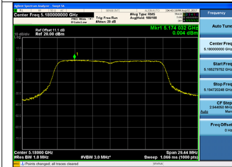
802.11n_HT20 UNII 1 BAND PSD CH 36
