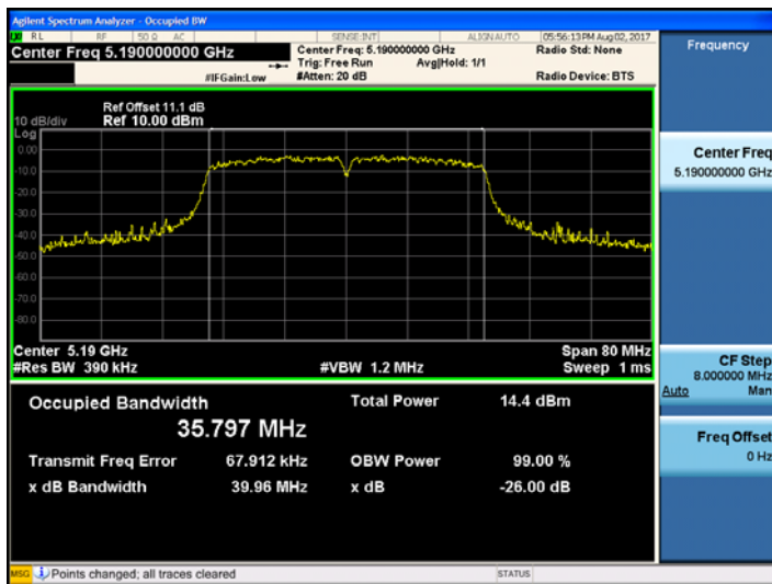
802.11ac_VHT40 UNII 1 BAND 26dB Bandwidth(CH 38)
