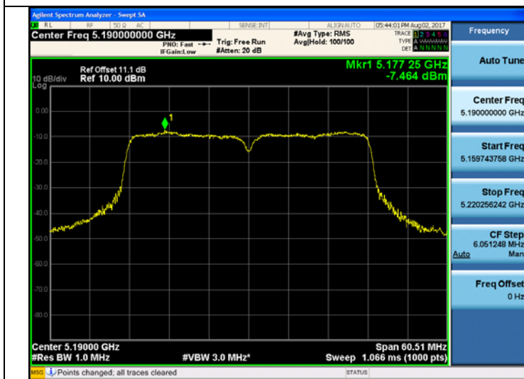
802.11n_HT40 UNII 1 BAND PSD CH 38
