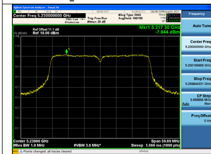
802.11ac_VHT40 UNII 1 BAND PSD CH 46
