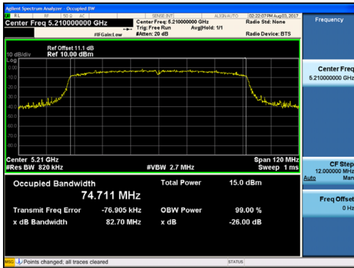
802.11ac_VHT80 UNII 1 BAND 26dB Bandwidth(CH 42)
