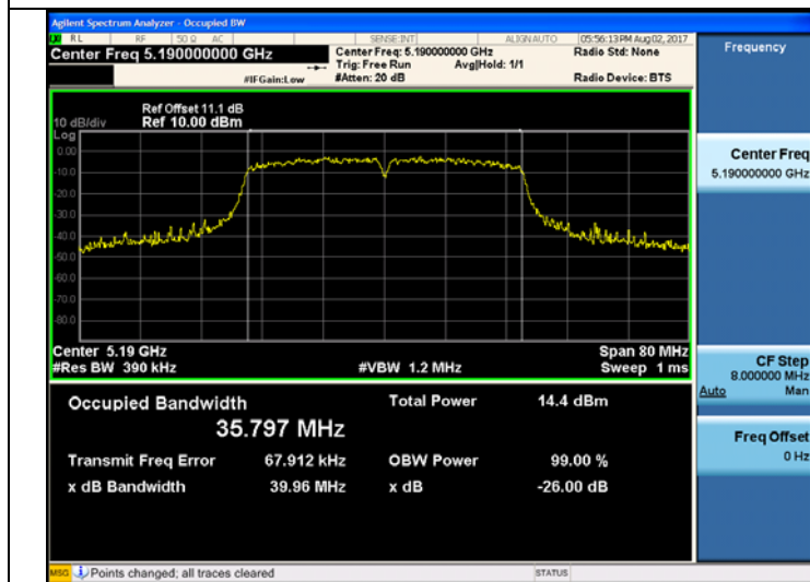
802.11ac_VHT40 UNII 1 BAND 99% Bandwidth(CH 38)
