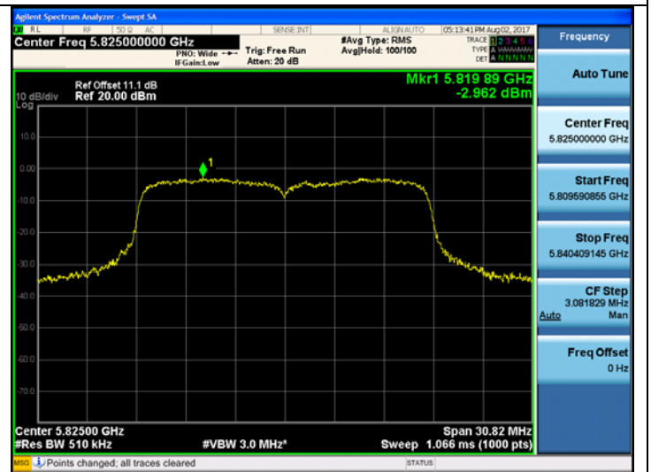
802.11n_HT20 UNII 3 BAND PSD CH 165
