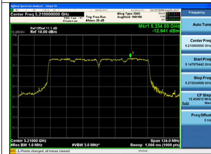
802.11ac_VHT80 UNII 1 BAND PSD CH 42
