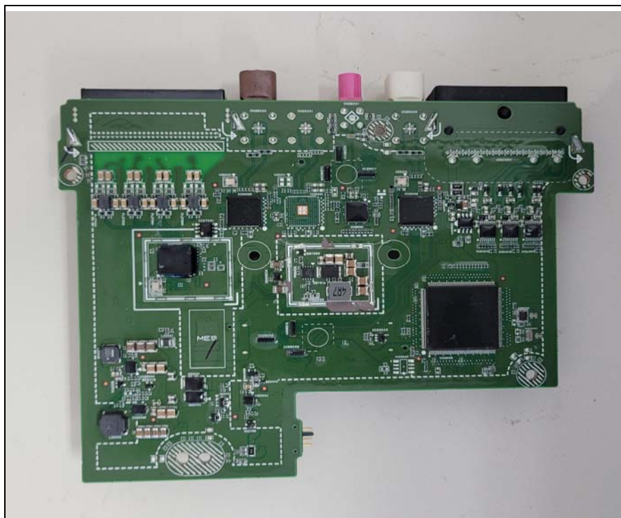
Bottom view of Sub PCB1
