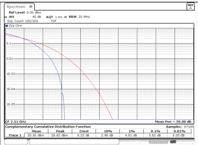
20 MHz 16QAM Low Channel – Full RB
