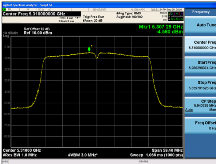
802.11n_HT40 UNII 2A BAND PSD CH 62_Internal Ant
