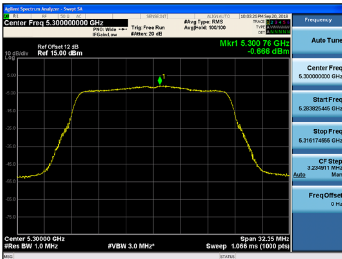
802.11ac_VHT20 UNII 2A BAND PSD CH 60_Internal Ant
