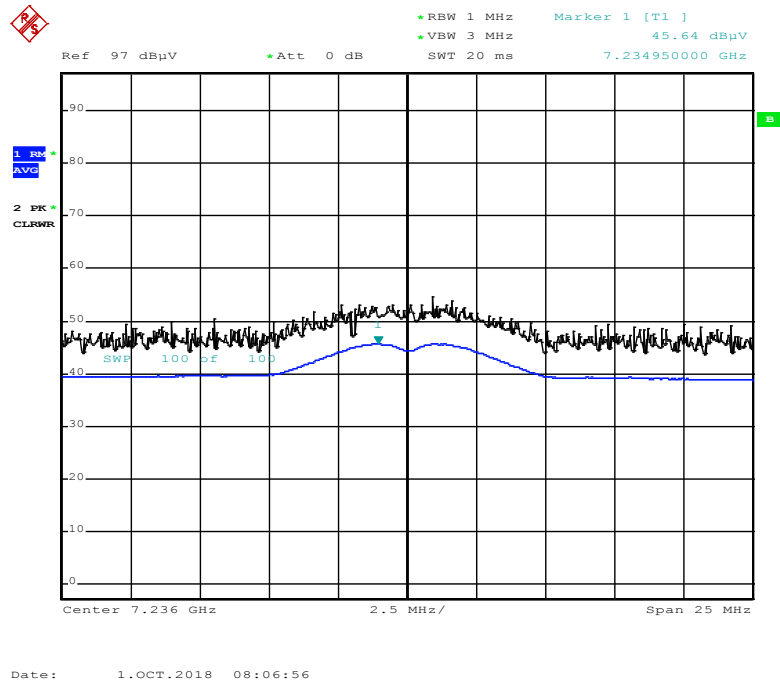
Radiated Spurious Emissions plot – Average Reading (802.11b, Ch.1 3rd Harmonic)
