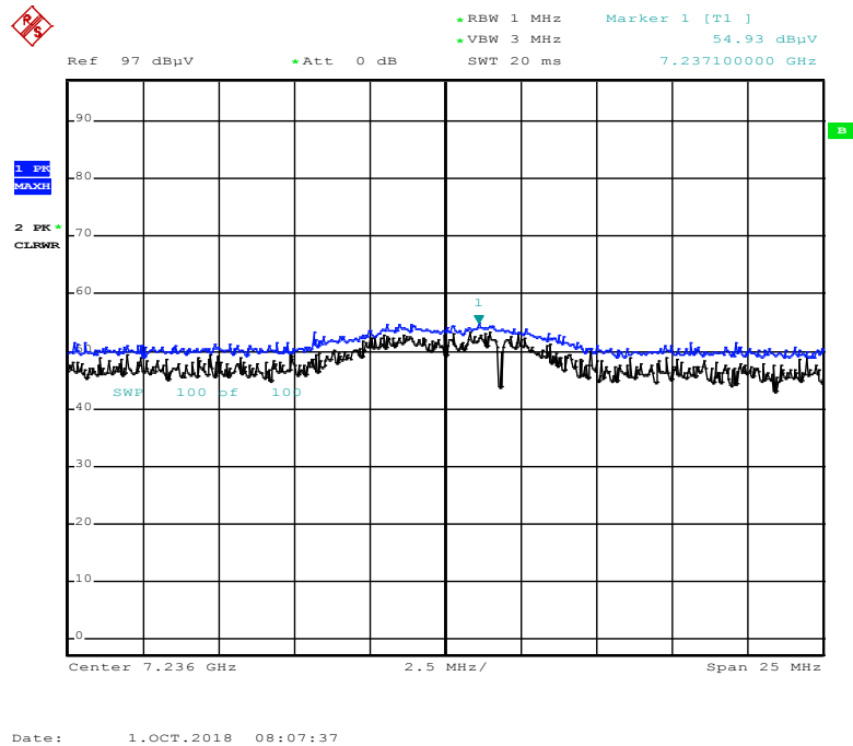
Radiated Spurious Emissions plot – Peak Reading (802.11b, Ch.1 3rd Harmonic)
