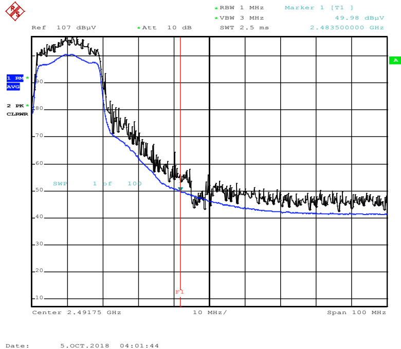
Radiated Restricted Band Edges plot – Average Reading (802.11n Ch.9)
