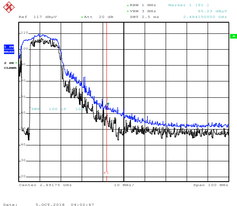
Radiated Restricted Band Edges plot – Peak Reading (802.11n Ch.9)
