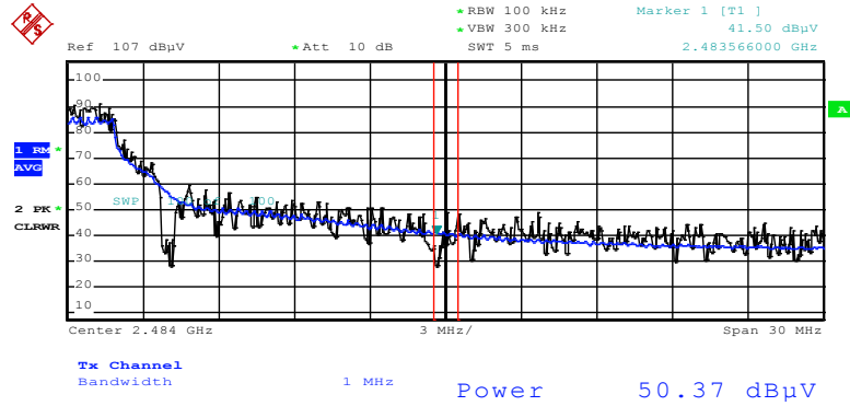
Radiated Restricted Band Edges plot – Average Reading (802.11n Ch.11)
