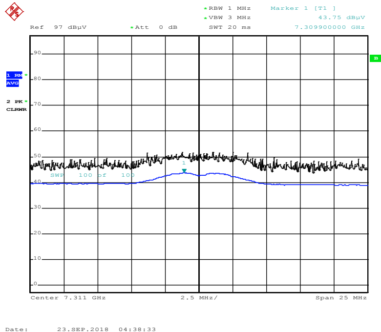
Radiated Spurious Emissions plot – Average Reading (802.11b, Ch.6 3rd Harmonic)
