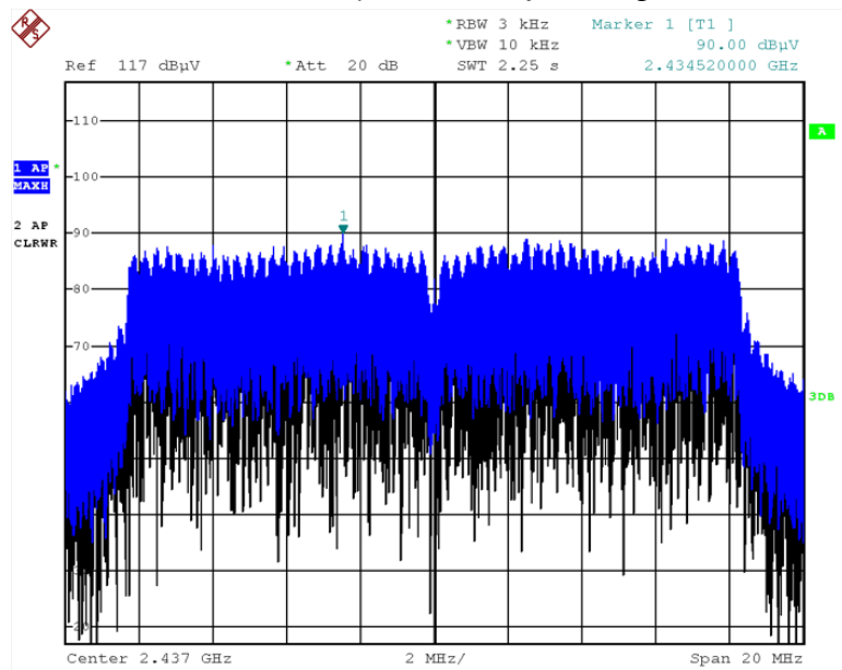
Radiated Power Spectral Density (802.11g, Ch.6)
