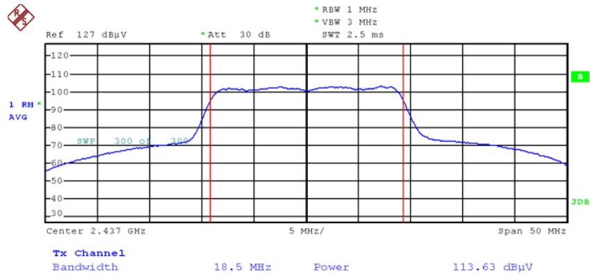
Radiated Output Power plot – (802.11n, Ch.6)
