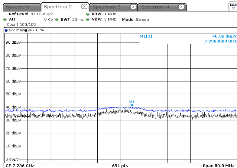
Radiated Spurious Emissions plot – Peak Measured Value
