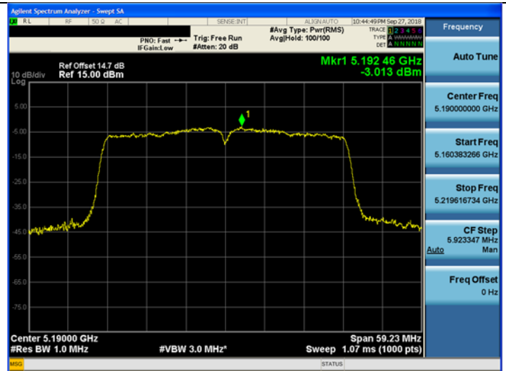
802.11n_HT40 UNII 1 BAND PSD CH 38_External Ant
