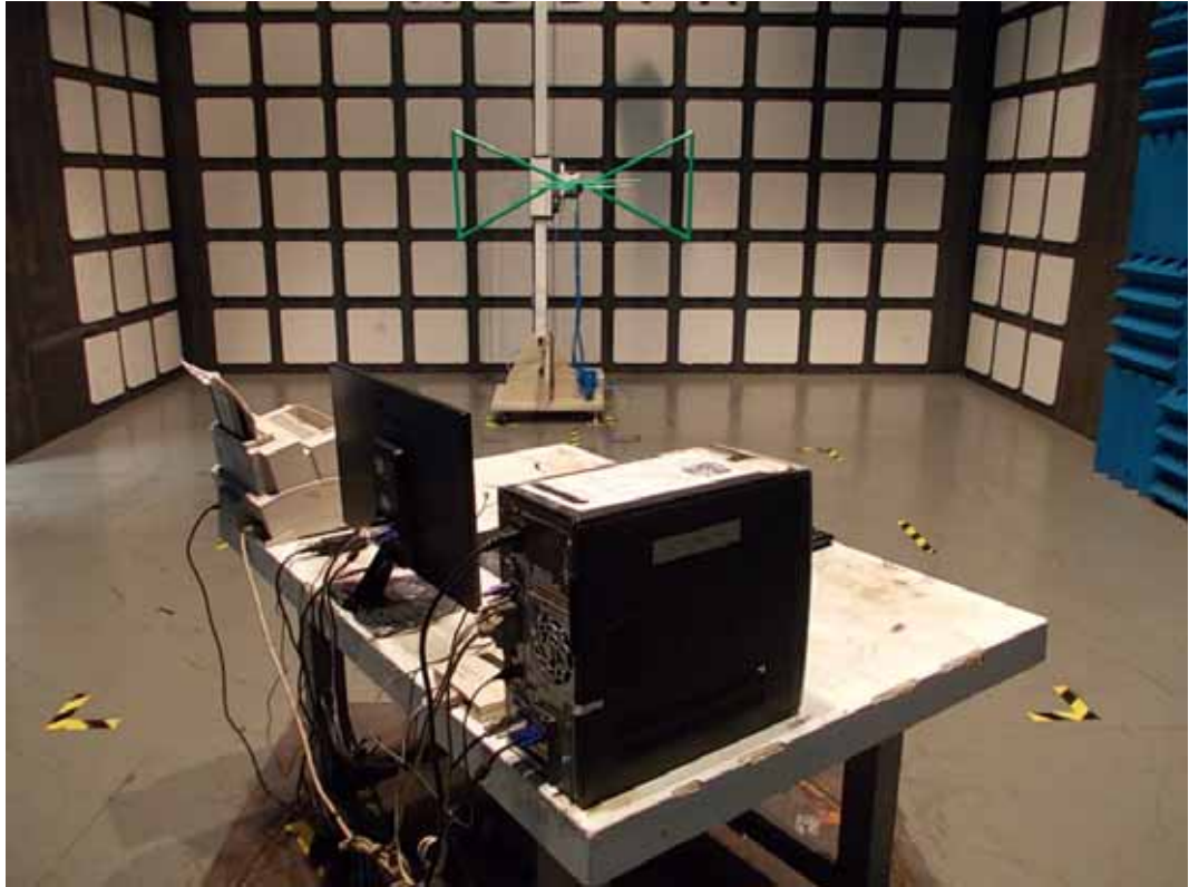
SETUP WITH MAXIMUM DETECTED EMISSION AT HORIZONTAL POLARIZATION (TEST MODE: DVI 640*480@60Hz, ADAPTER #3)
