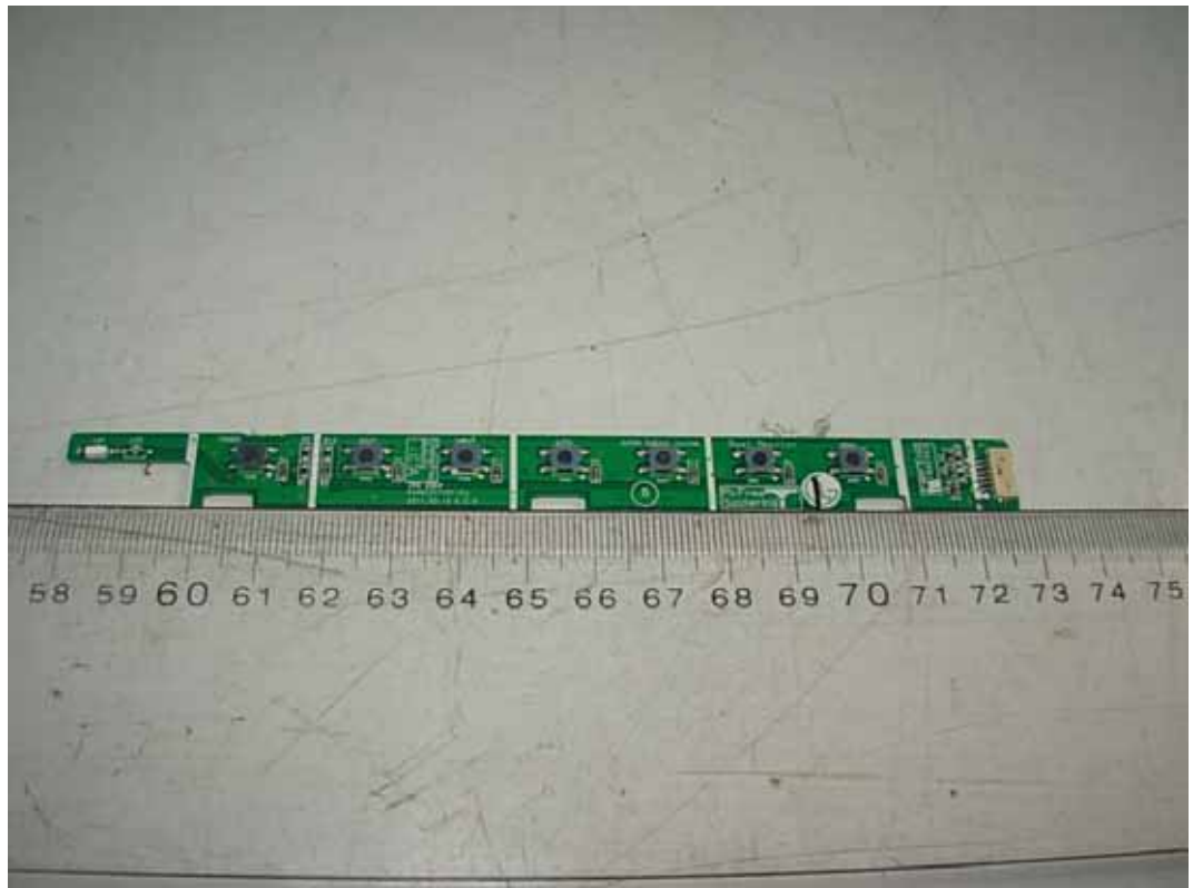
FIGURE 10 LCD MONITOR (M/N: IPS235VX) KEY BOARD (COMPONENT SIDE)
