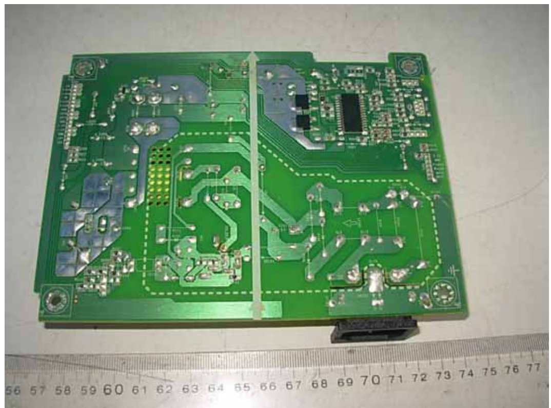
FIGURE 7 LCD MONITOR (M/N: IPS235VX) POWER BOARD (SOLDERED SIDE)
