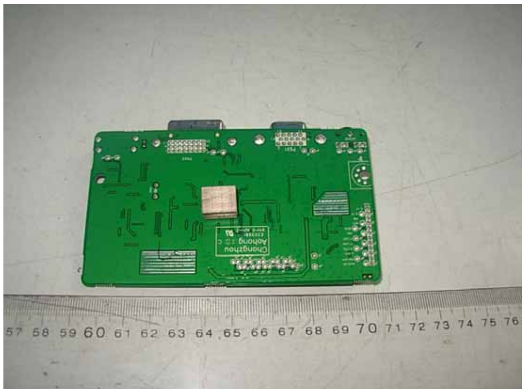
FIGURE 4 LCD MONITOR (M/N: IPS235VX) MAIN BOARD (COMPONENT SIDE)
