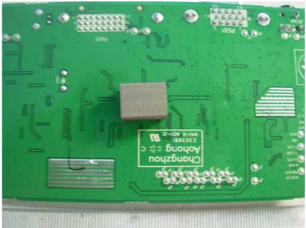
FIGURE 12 LCD MONITOR (M/N: IPS235VX) DEBUG #1
