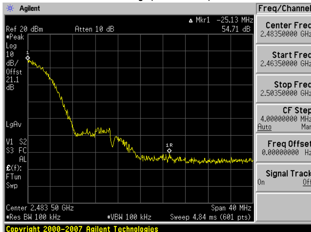
BandEdge (802.11b-CH11)
