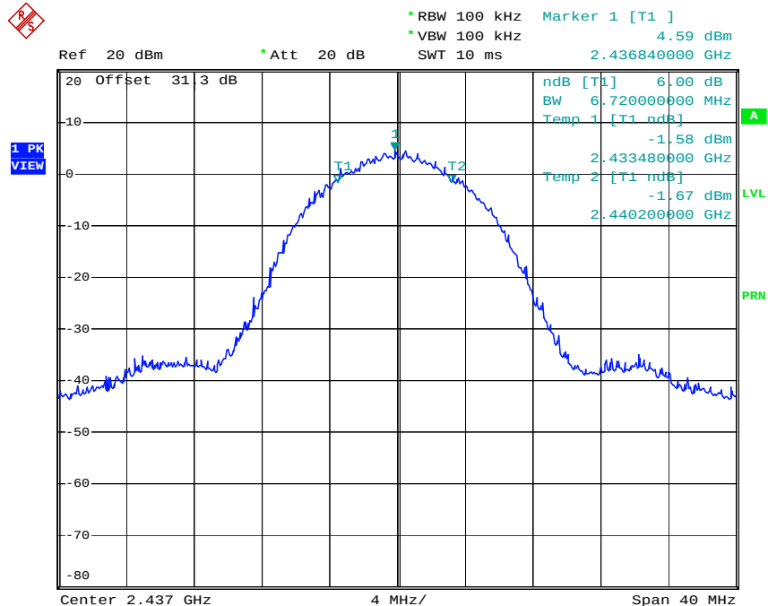
6dB Bandwidth plot (802.11b-CH 6)
