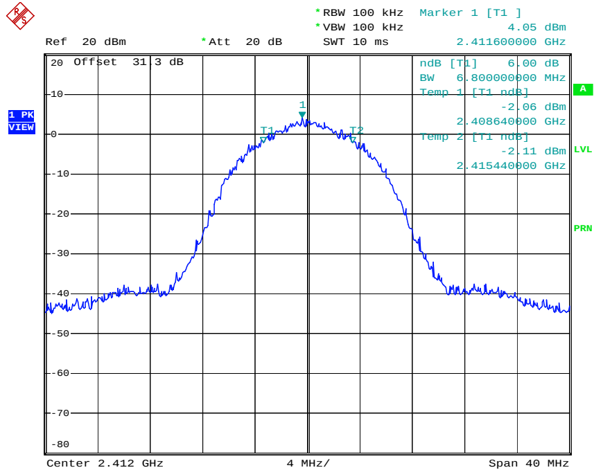
6dB Bandwidth plot (802.11b-CH 1)
