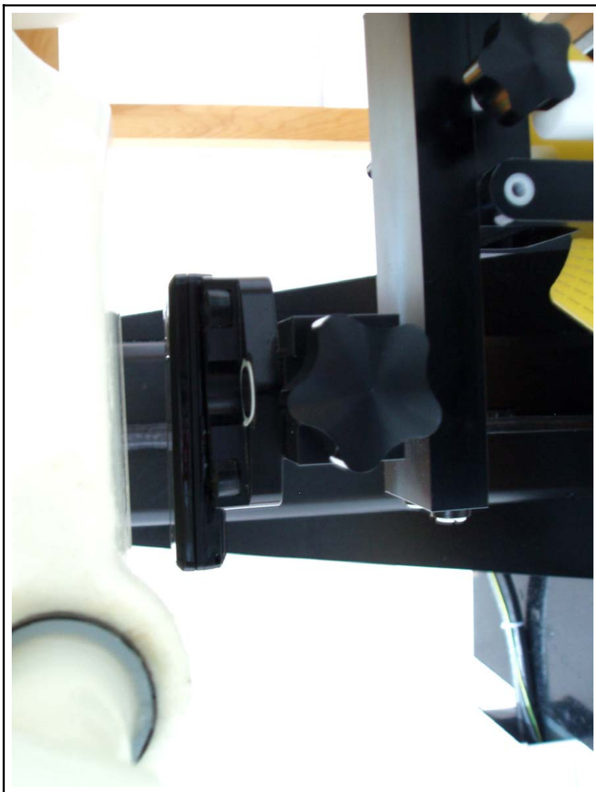
Figure 10 Body SAR Test Setup – w/o Holster
