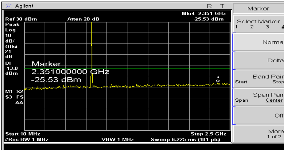
PLOTS OF EMISSION (EDGE): Out of Band(Ch128)
