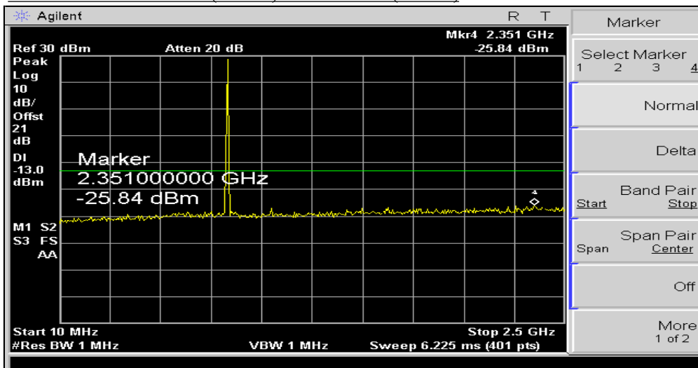
PLOTS OF EMISSION (EDGE): Out of Band(Ch190)
