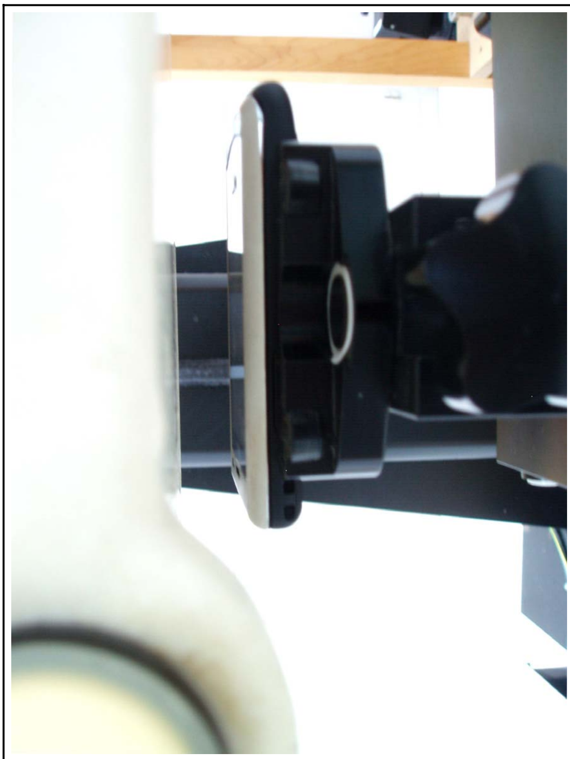
Figure 9 Body SAR Test Setup – w/o Holster
