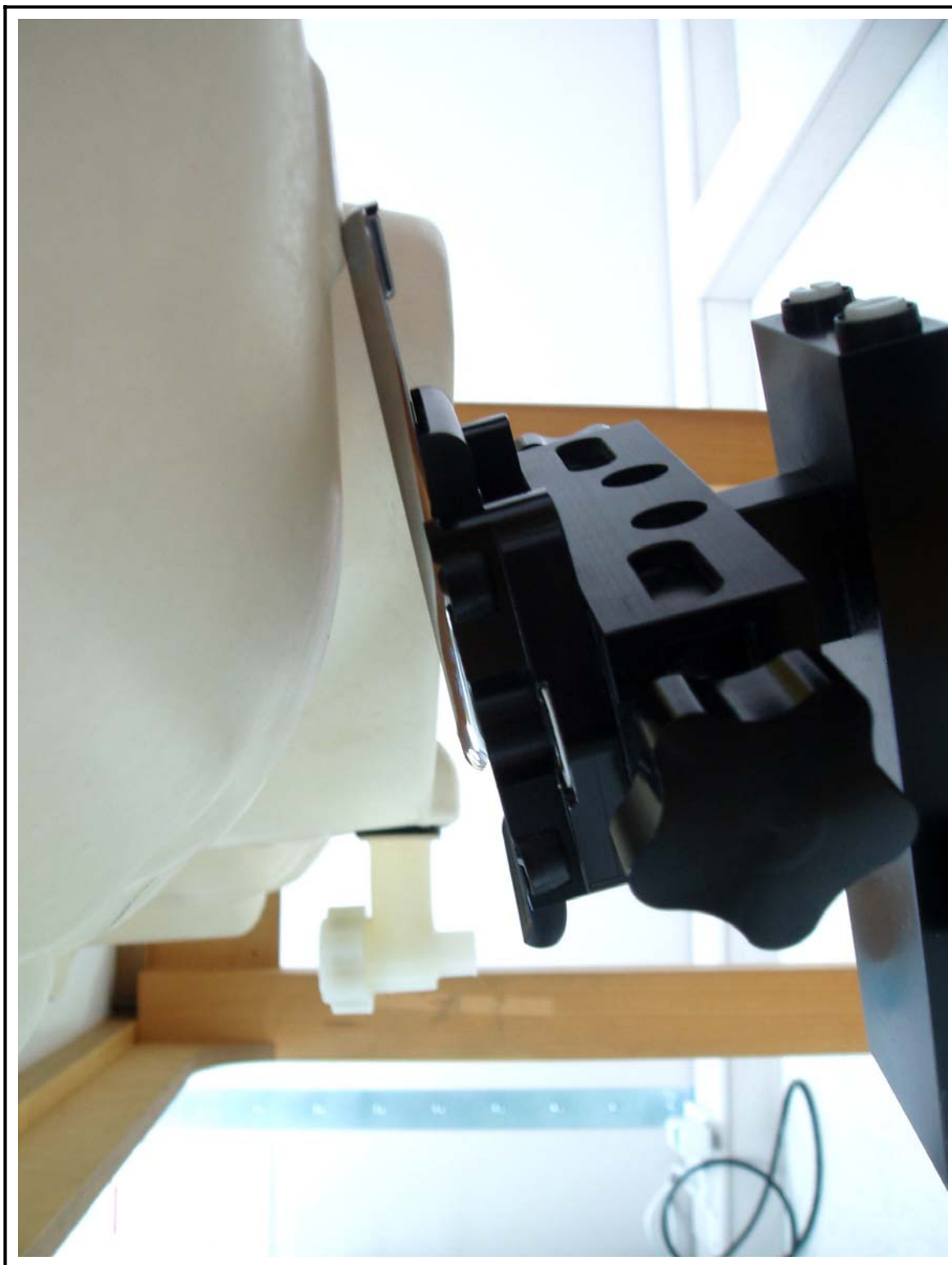
Figure 8 Left Head SAR Test Setup – Ear Tilt Position
