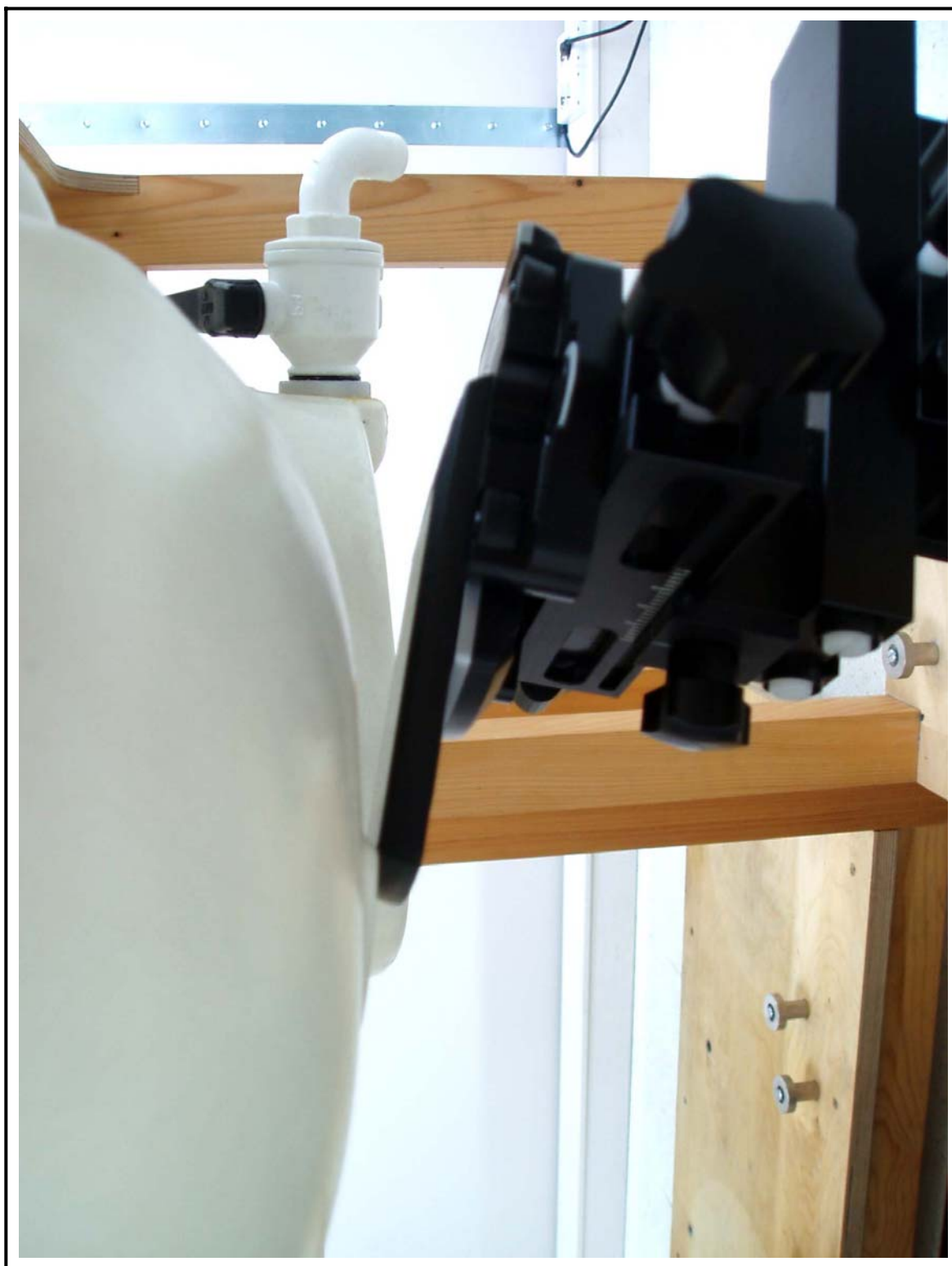
Figure 12 Right Head SAR Test Setup - Cheek Tilt Position
