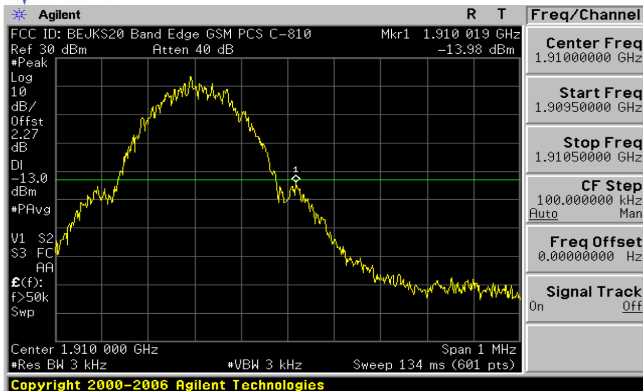
Plot 7-9. Band Edge Plot (PCS GSM Mode – Ch. 810)
