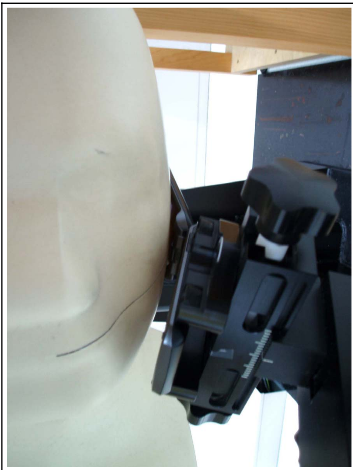
Figure 8 Left Head SAR Test Setup - Cheek Touch Position
