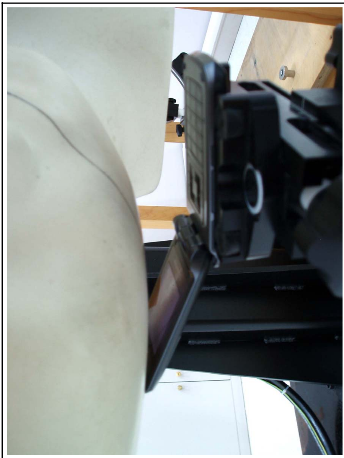
Figure 5 Right Head SAR Test Setup – Ear Tilt Position
