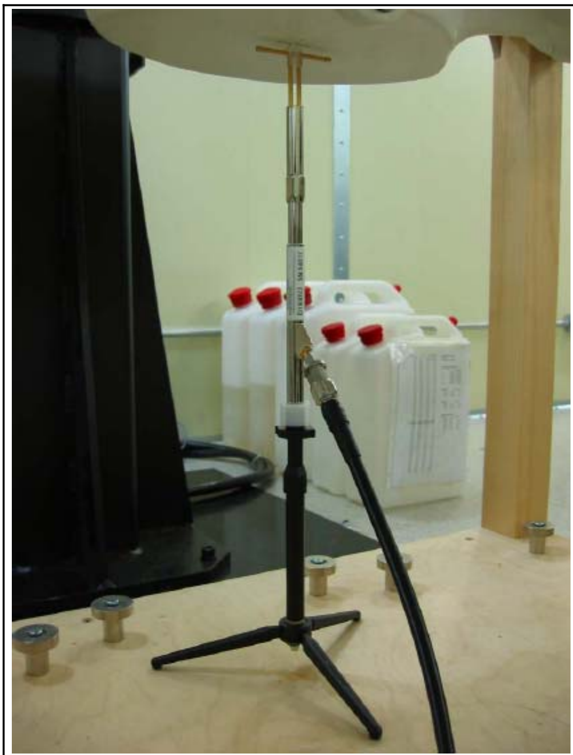
Figure 1 1900 MHz Dipole Validation Test Setup
