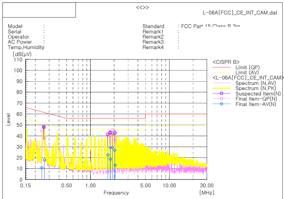
Plot 7-1. Line-Conducted Test Plot.
