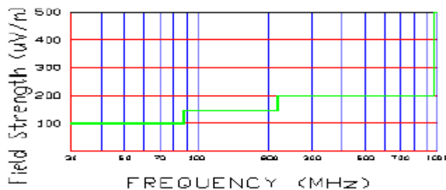
Figure 7-1. 3 Meter Limits
