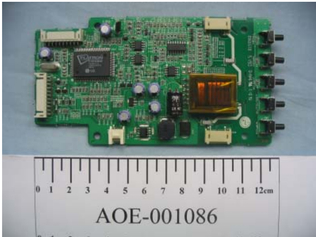
FIGURE 8 LCD MONITOR (M/N: L1552SQ) MAIN BOARD (COMPONENT SIDE)
