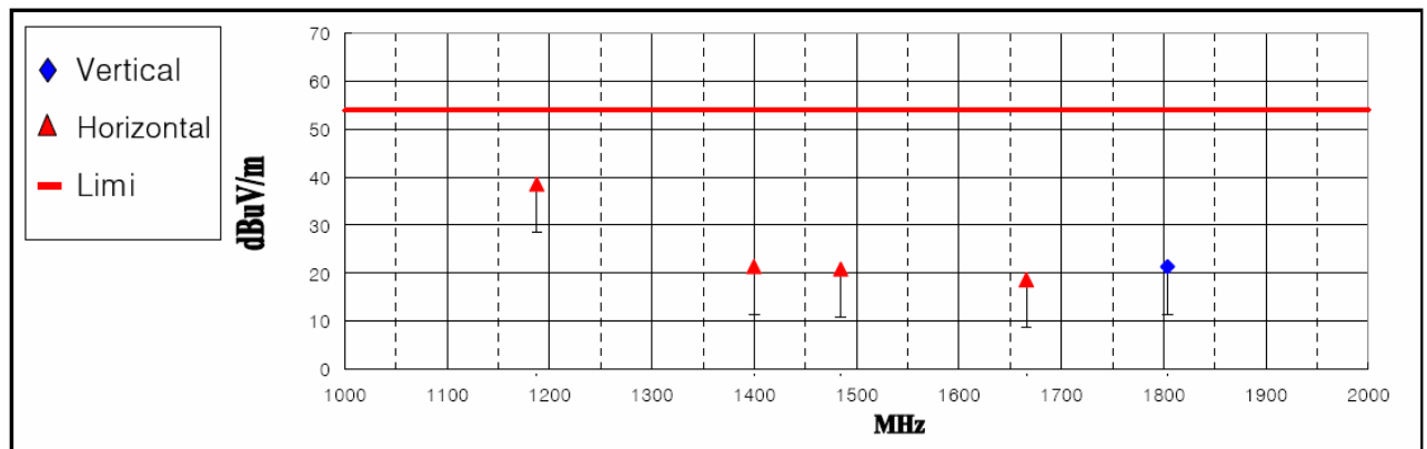
< Fig 5. Radiated Emission _ Analog (1000MHz ~ 2000MHz) >
