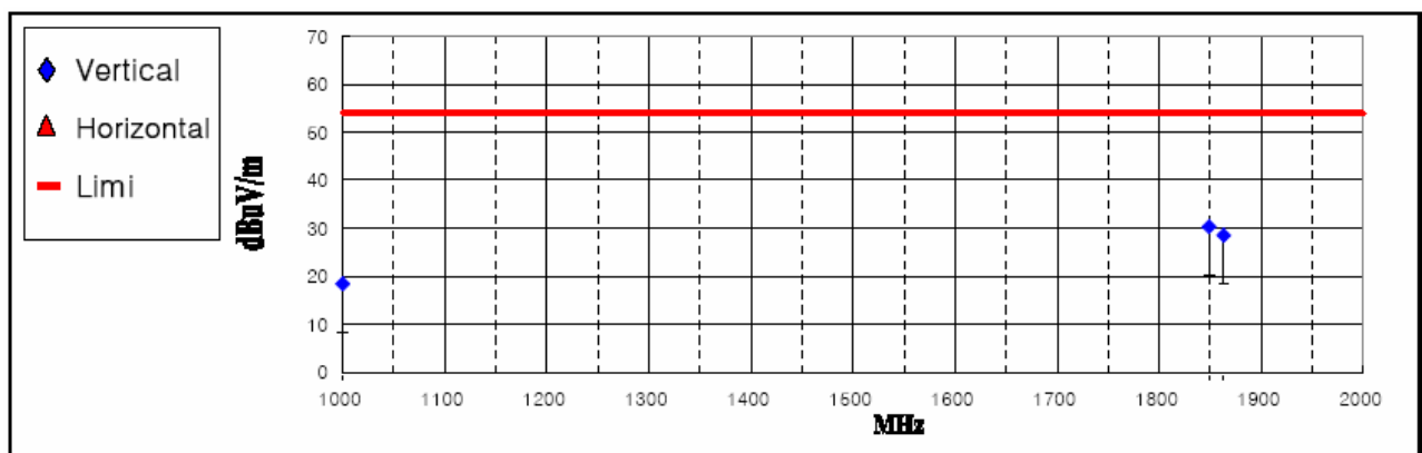
< Fig 5. Radiated Emission (1000MHz ~ 2000MHz) >
