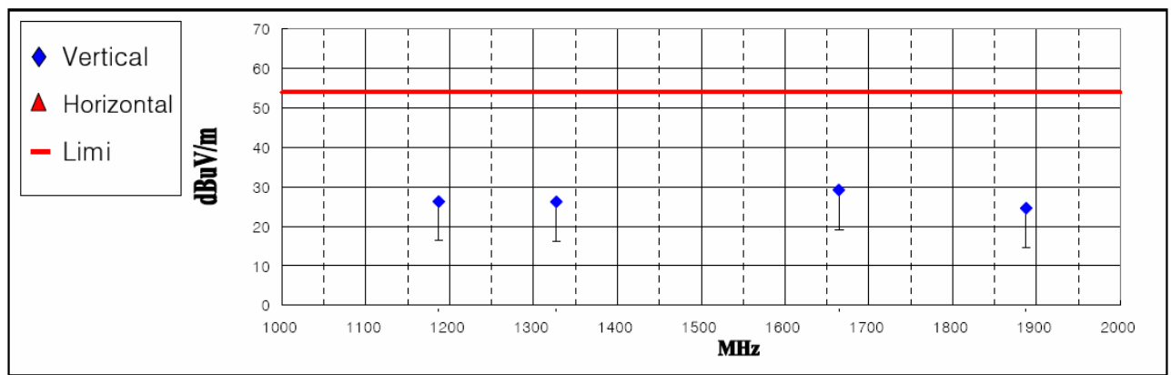
< Fig 5. Radiated emission result (1000MHz ~ 2000MHz)>
