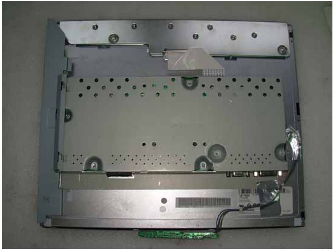
FIGURE 1 LCD MONITOR (M/N: L1742PEU) COVER REMOVED
