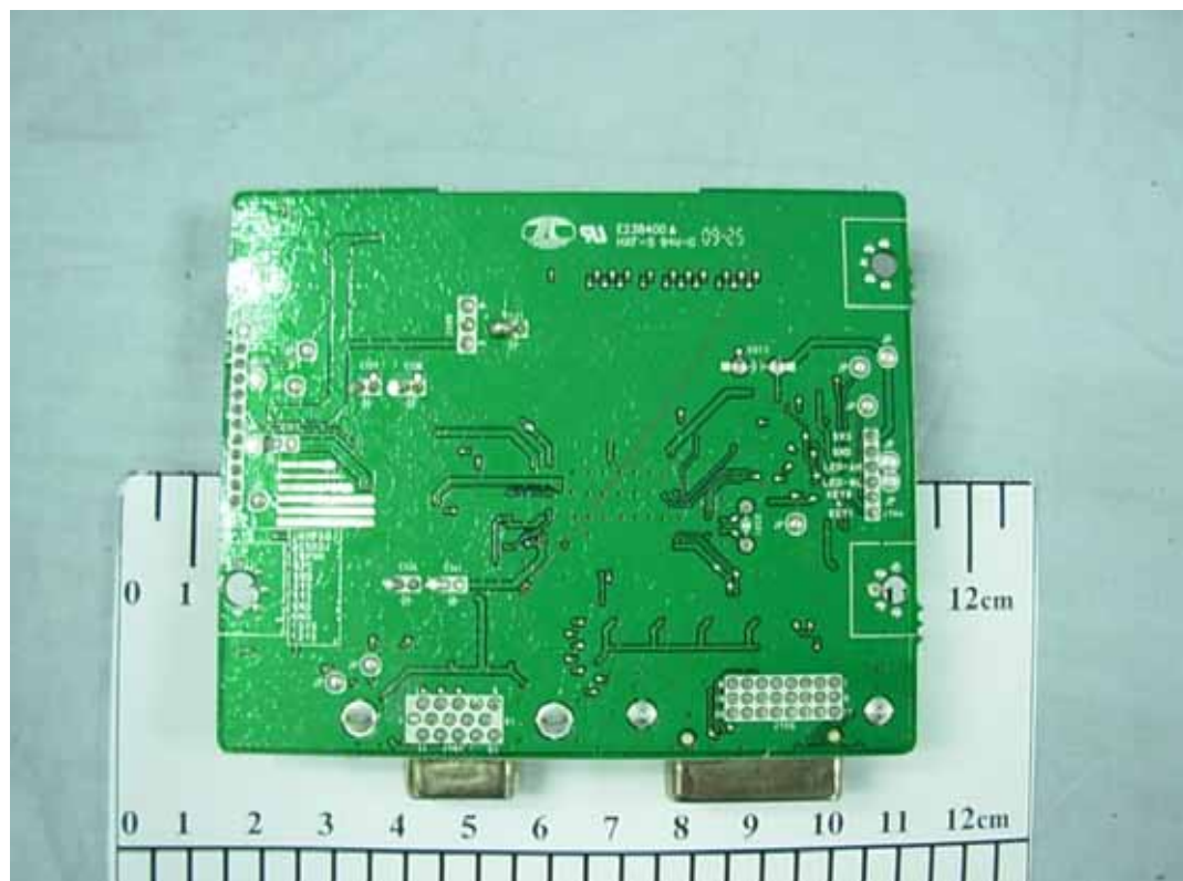
FIGURE 3 LCD MONITOR (M/N: L1742PEU) MAIN BOARD (SOLDERED SIDE)
