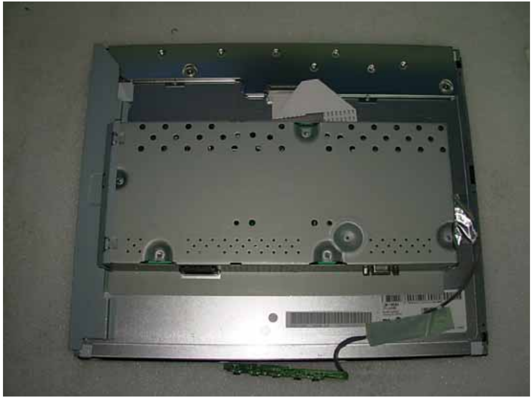
FIGURE 14 LCD MONITOR (M/N: L1742SEU) COVER REMOVED
