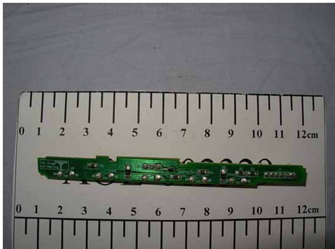
FIGURE 11 LCD MONITOR (M/N: L1742PEU) BUTTON BOARD (SOLDERED SIDE)
