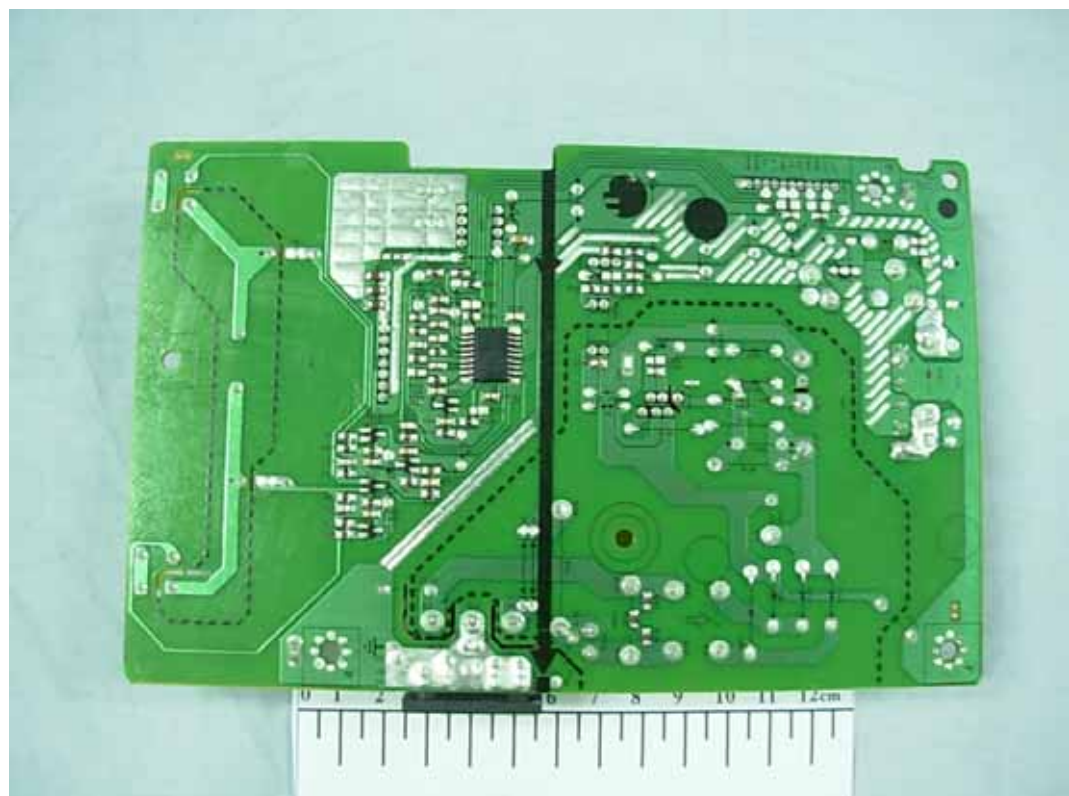
FIGURE 7 LCD MONITOR (M/N: L1742PEU) POWER BOARD (SOLDERED SIDE)
