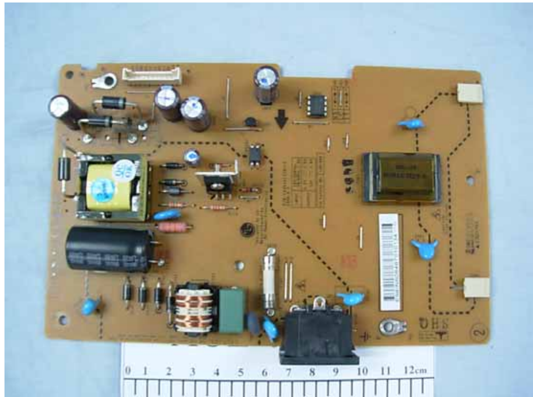
FIGURE 19 LCD MONITOR (M/N: L1742SEU) POWER BOARD (COMPONENT SIDE)
