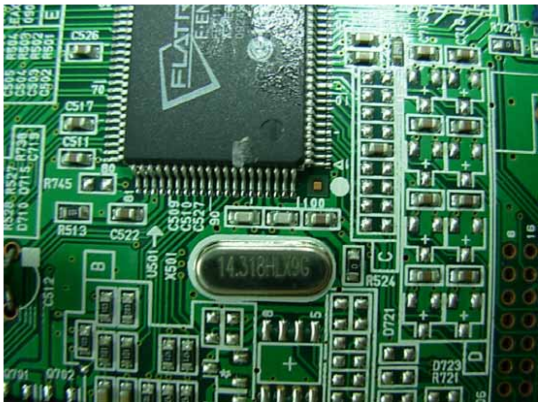
FIGURE 18 LCD MONITOR (M/N: L1742SEU) CRYSTAL
