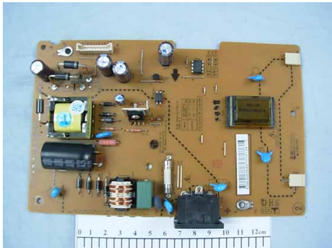
FIGURE 6 LCD MONITOR (M/N: L1742PEU) POWER BOARD (COMPONENT SIDE)
