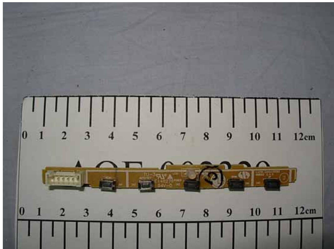
FIGURE 23 LCD MONITOR (M/N: L1742SEU) BUTTON BOARD (COMPONENT SIDE)
