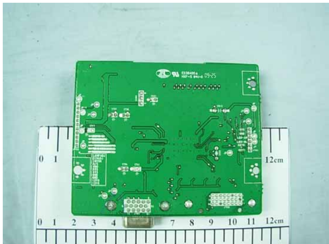
FIGURE 16 LCD MONITOR (M/N: L1742SEU) MAIN BOARD (SOLDERED SIDE)
