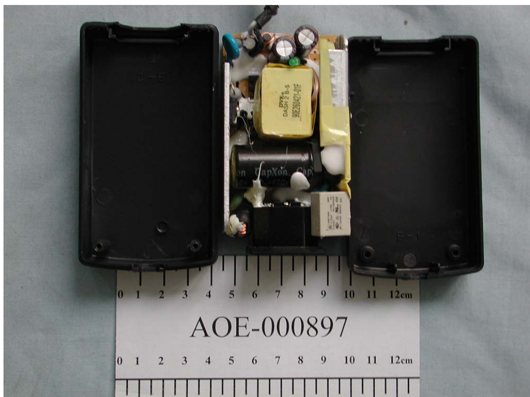
FIGURE 18 LCD MONITOR (M/N: L1750UN) ADAPTOR (COVER REMOVED)
