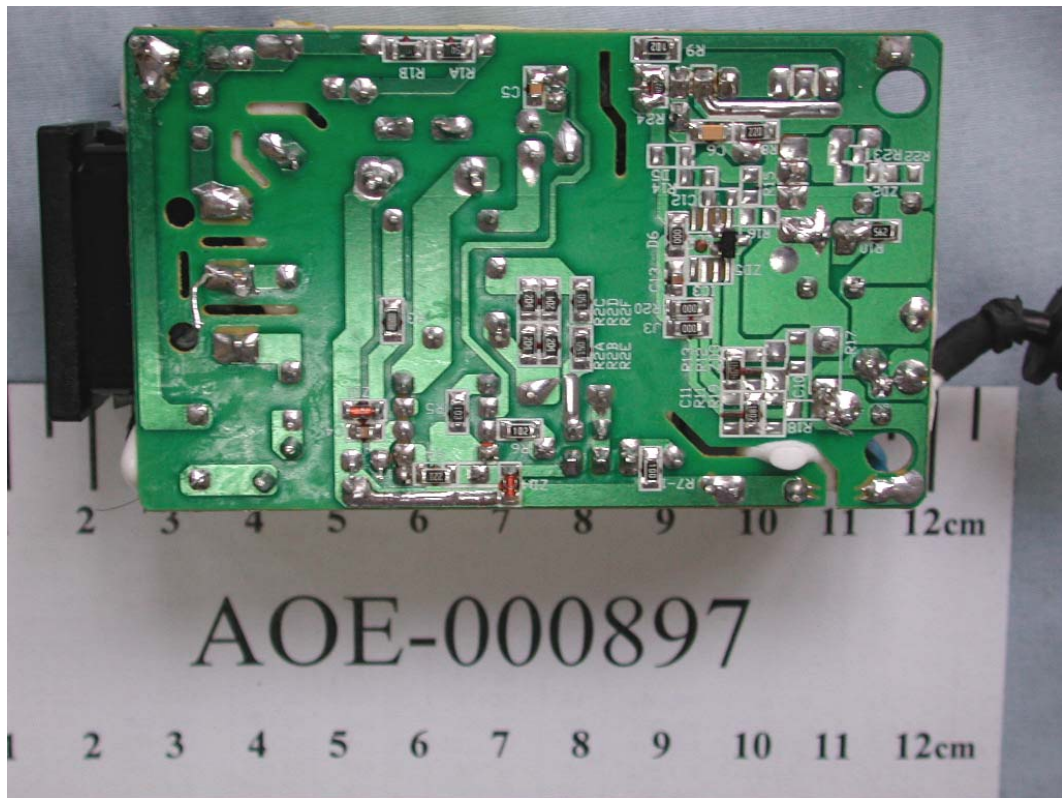
FIGURE 21 LCD MONITOR (M/N: L1750UN) ADAPTOR (SOLDERED SIDE 2)
