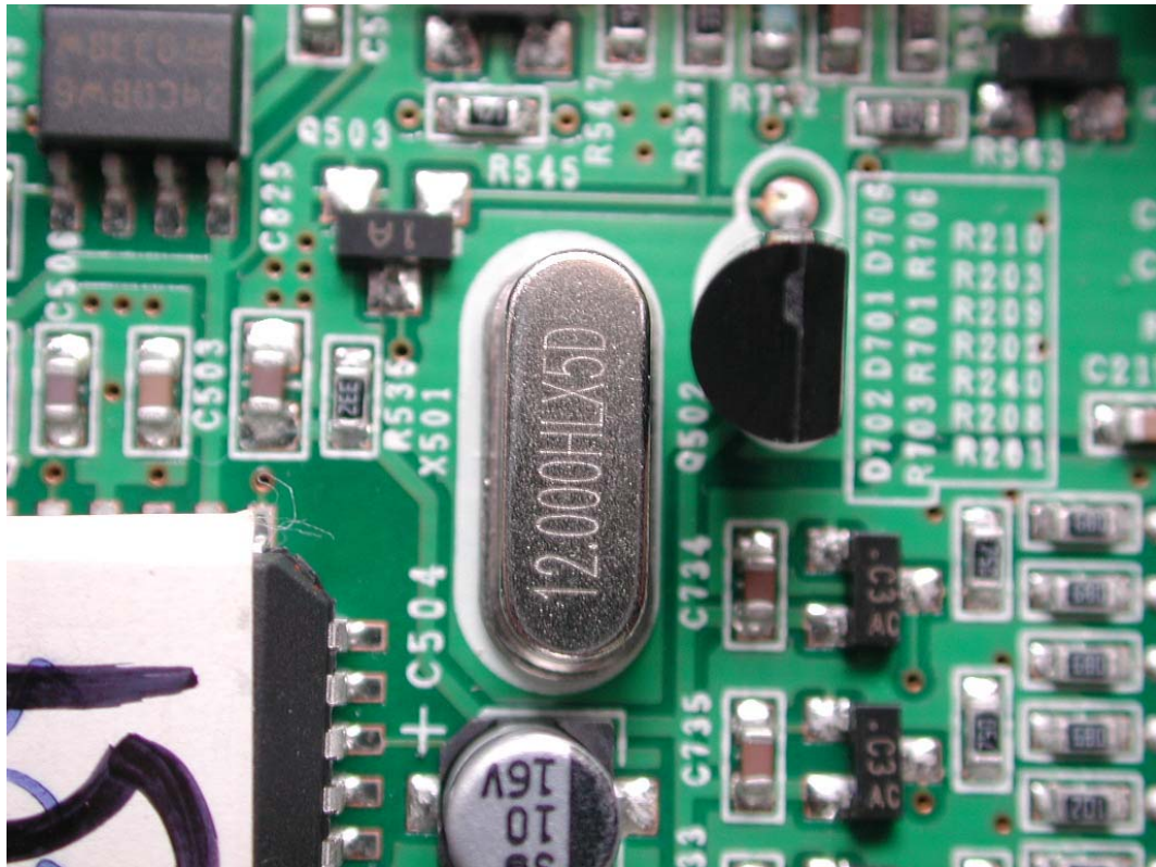
FIGURE 5 LCD MONITOR (M/N: L1750UN) MAIN CRYSTAL
