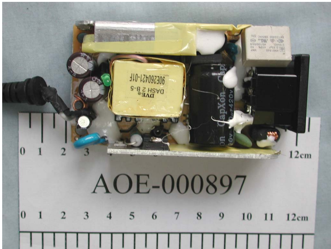
FIGURE 19 LCD MONITOR (M/N: L1750UN) ADAPTOR (COMPONENT SIDE)
