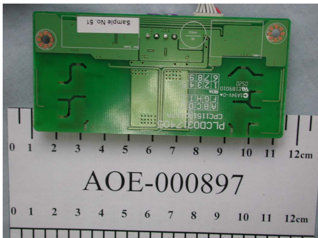
FIGURE 8 LCD MONITOR (M/N: L1750UN) INVERT BOARD (BACK VIEW)
