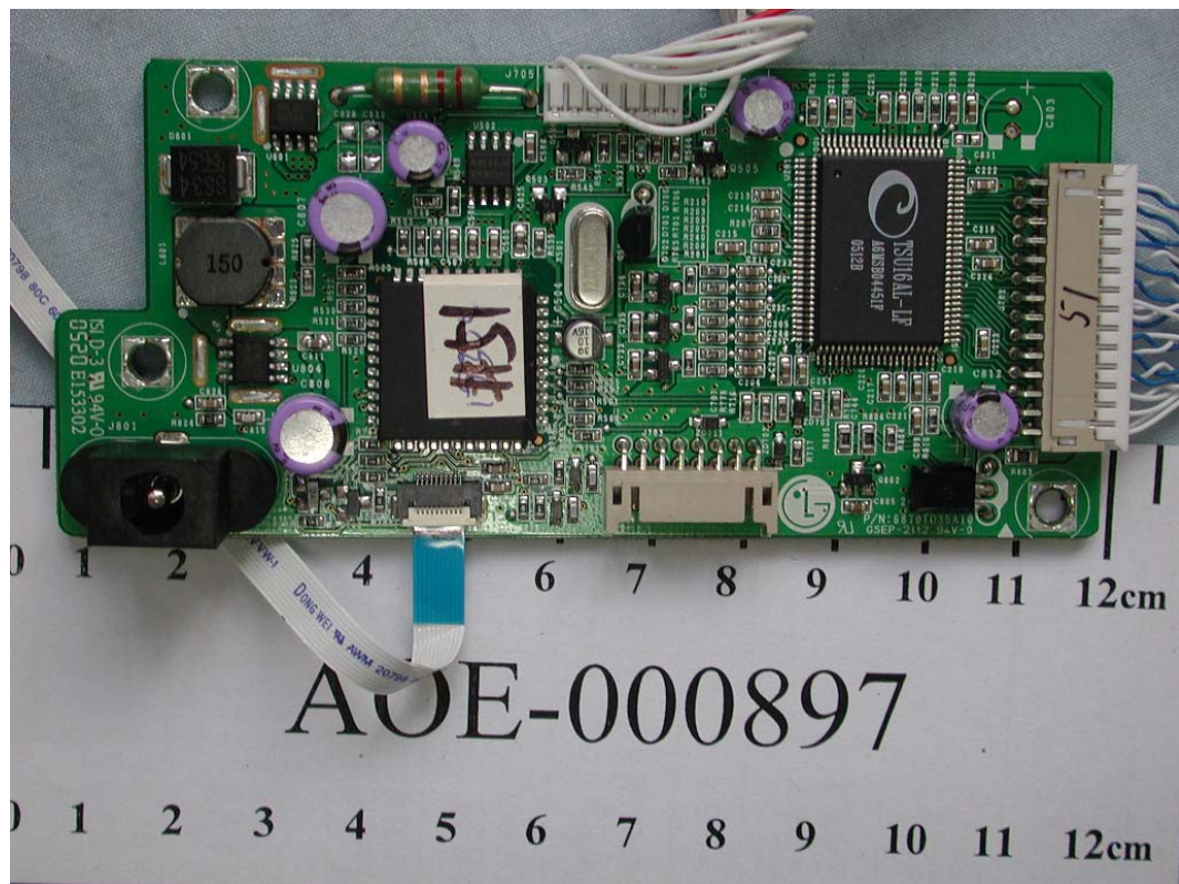
FIGURE 3 LCD MONITOR (M/N: L1750UN) MAIN BOARD (COMPONENT SIDE)
