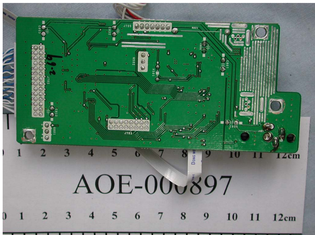
FIGURE 4 LCD MONITOR (M/N: L1750UN) MAIN BOARD (SOLDERED SIDE)
