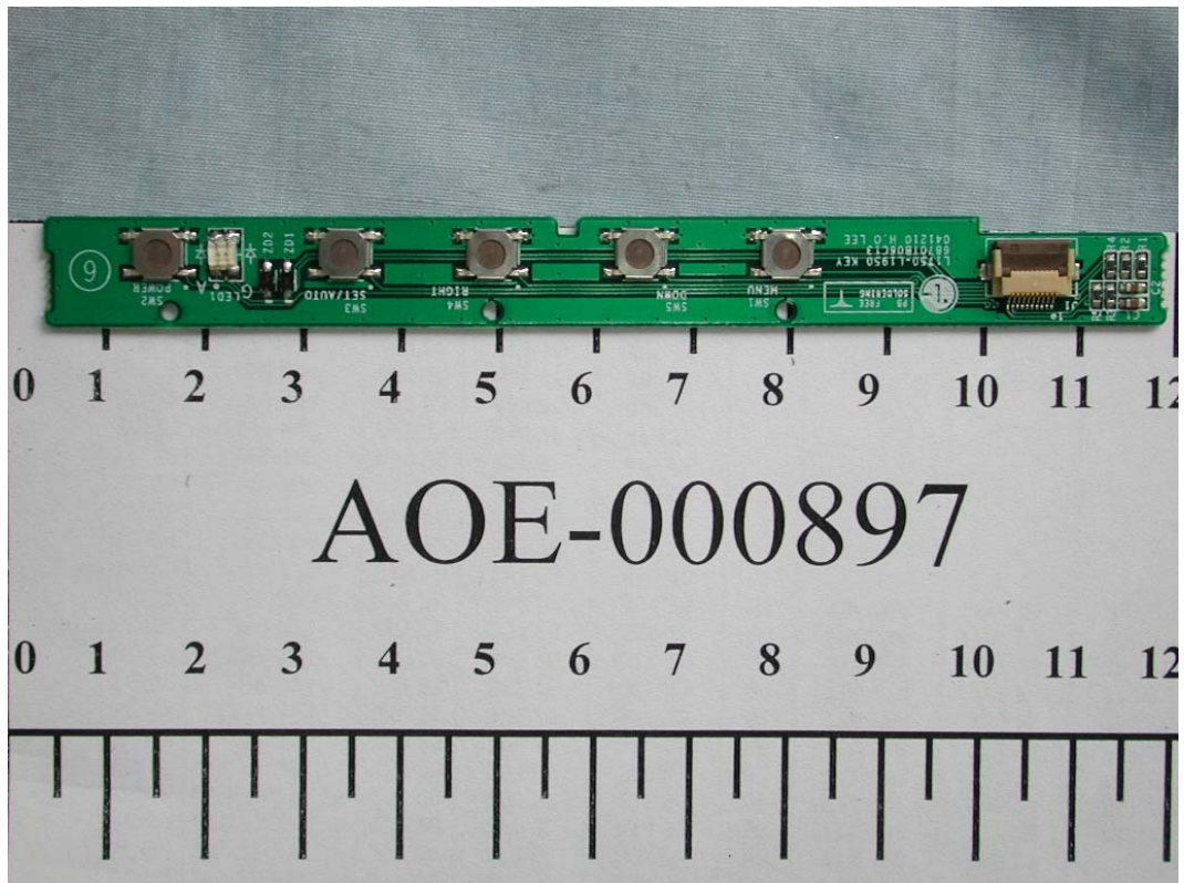
FIGURE 9 LCD MONITOR (M/N: L1750UN) OPERATION BOARD (FRONT VIEW)
