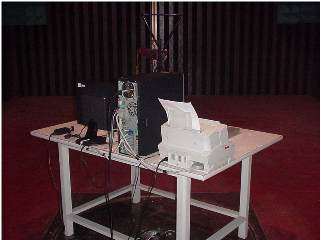
SETUP WITH MAXIMUM DETECTED EMISSION AT VERTICAL POLARIZATION (1280*1024 75Hz)
