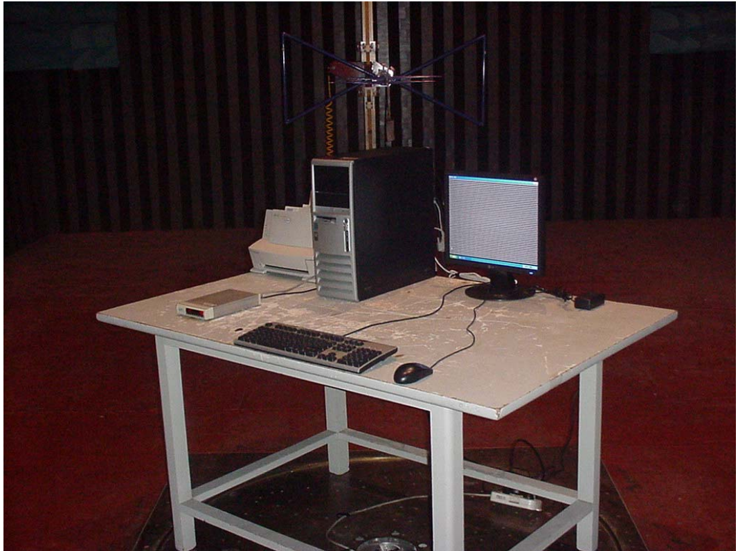
SETUP WITH MAXIMUM DETECTED EMISSION AT HORIZONTAL POLARIZATION (1280*1024 75Hz)
