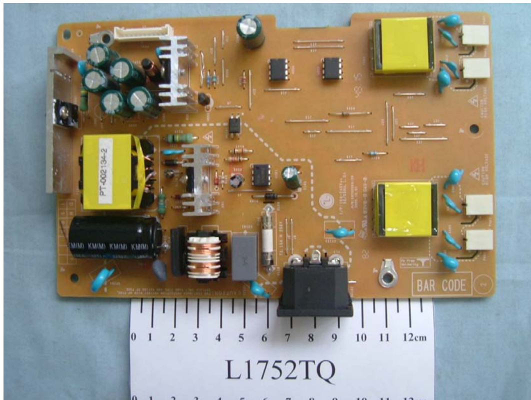
FIGURE 12 LCD MONITOR (M/N: L1752TQ) POWER BOARD (COMPONENT SIDE)
