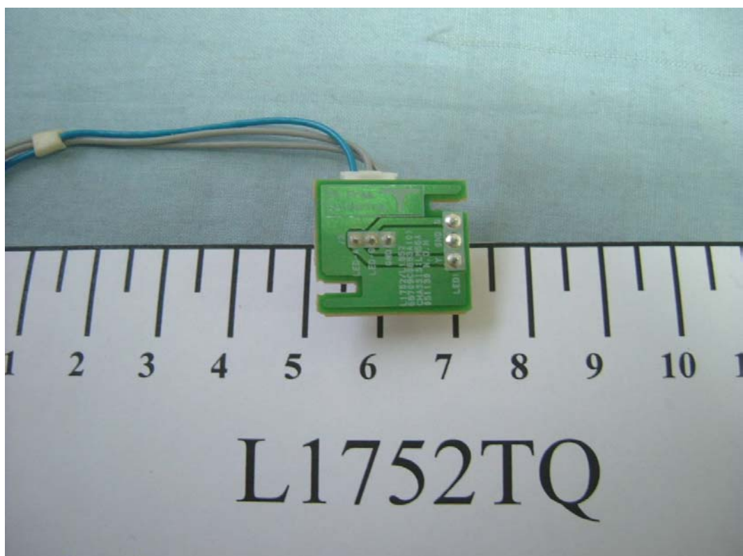
FIGURE 20 LCD MONITOR (M/N: L1752TQ) CONTROL BOARD 2 (SOLDERED SIDE)
