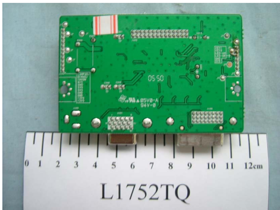
FIGURE 15 LCD MONITOR (M/N: L1752TQ) MAIN BOARD (SOLDERED SIDE)
