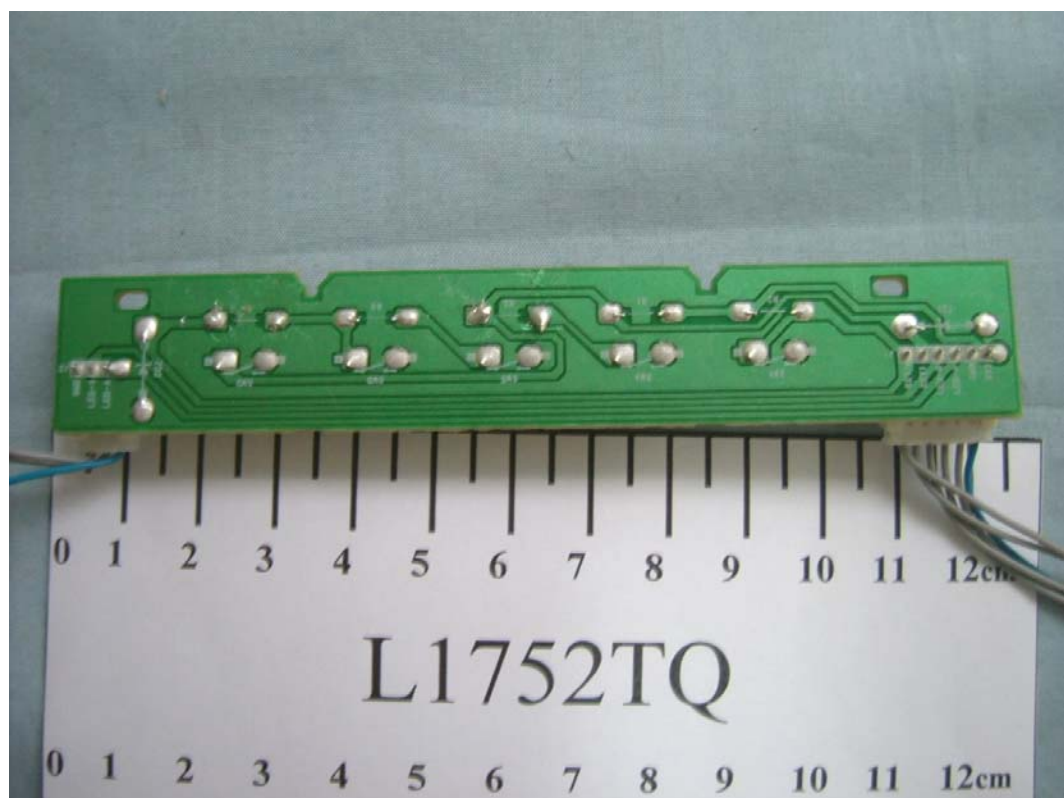
FIGURE 18 LCD MONITOR (M/N: L1752TQ) CONTROL BOARD 1 (SOLDERED SIDE)
