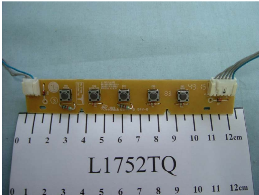
FIGURE 17 LCD MONITOR (M/N: L1752TQ) CONTROL BOARD 1 (COMPONENT SIDE)
