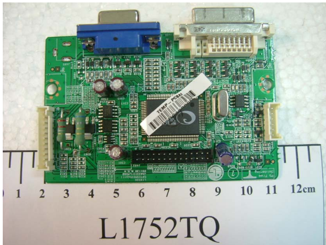
FIGURE 14 LCD MONITOR (M/N: L1752TQ) MAIN BOARD (COMPONENT SIDE)
