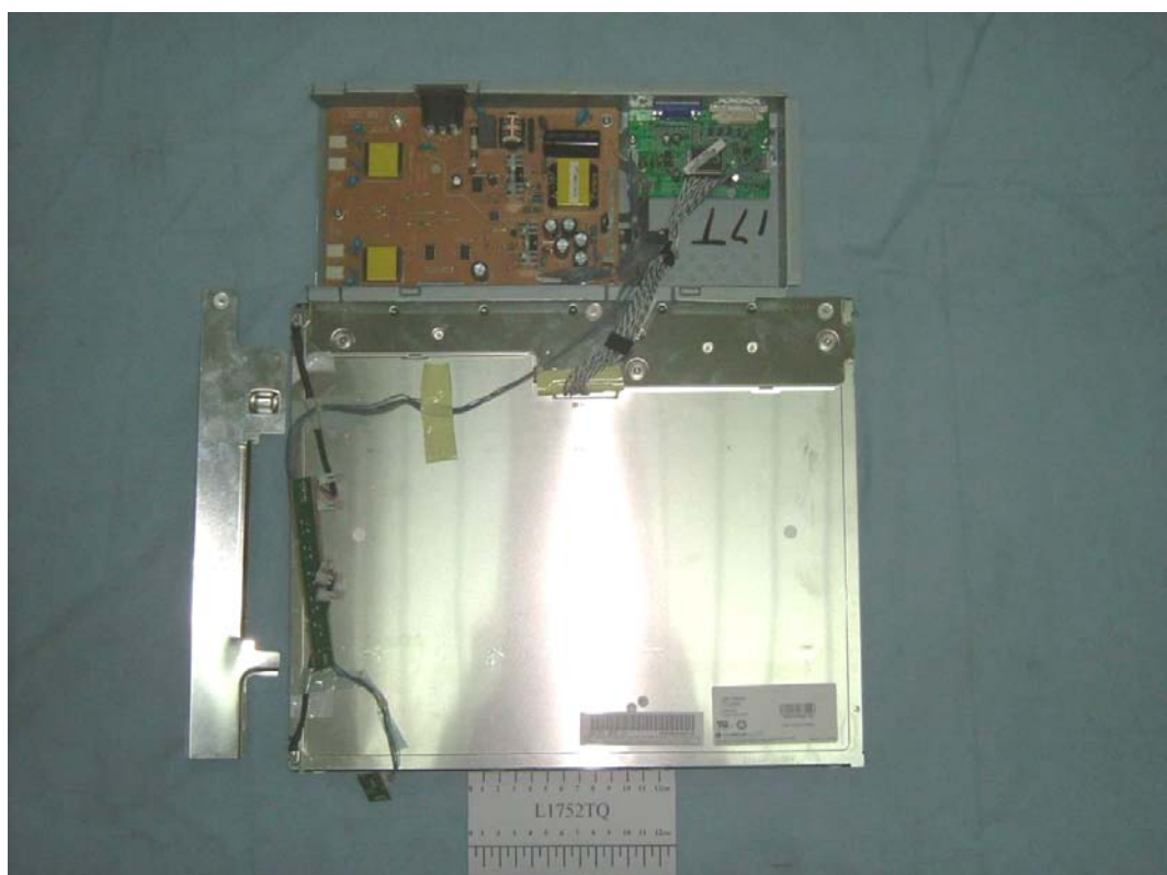
FIGURE 6 LCD MONITOR (M/N: L1752TQ) BOARDS REMOVED
