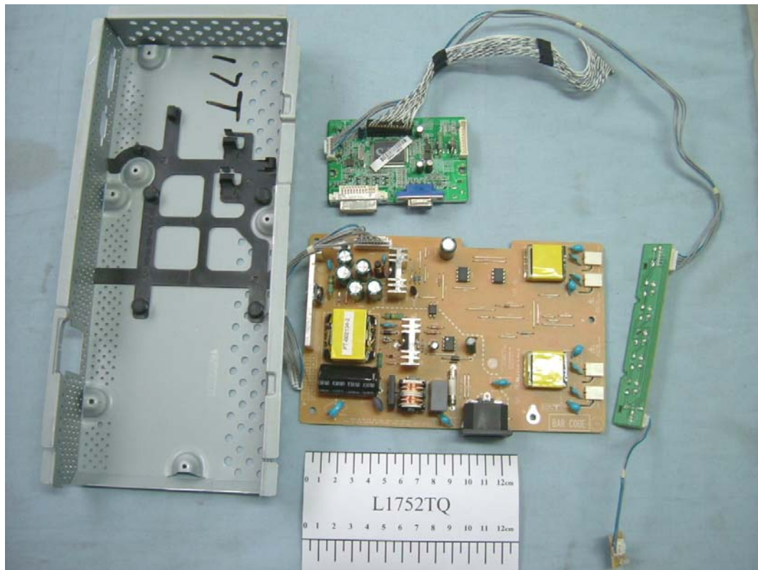
FIGURE 11 LCD MONITOR (M/N: L1752TQ) SHIELDED COVER REMOVED
