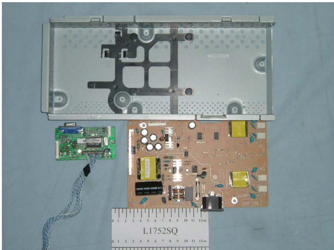
FIGURE 12 LCD MONITOR (M/N: L1752SQ) SHIELDED CASE INSIDE 2
