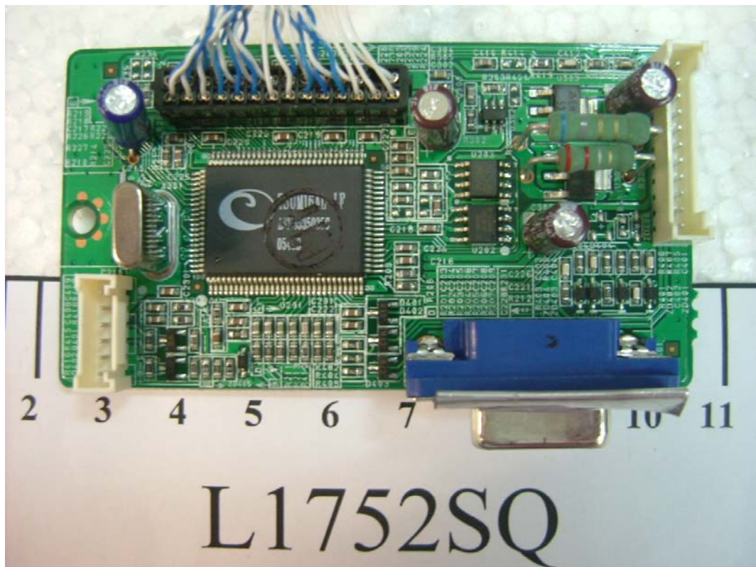
FIGURE 15 LCD MONITOR (M/N: L1752SQ) MAIN BOARD (COMPONENT SIDE)
