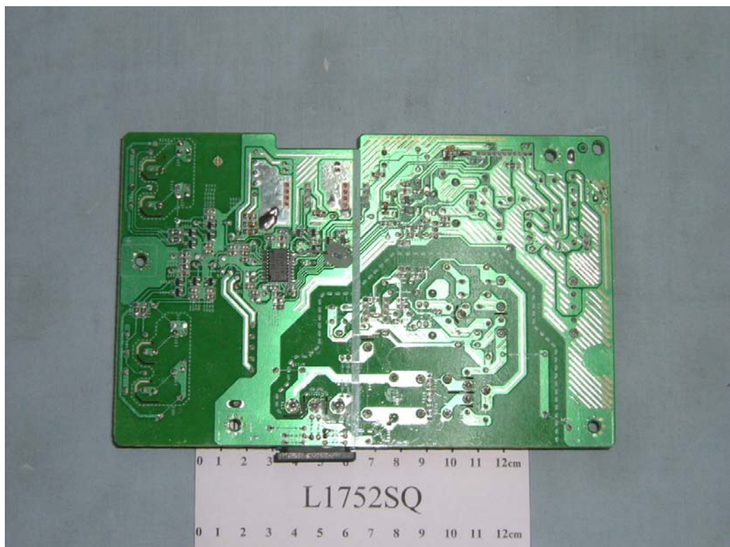
FIGURE 14 LCD MONITOR (M/N: L1752SQ) POWER BOARD (SOLDERED SIDE)
