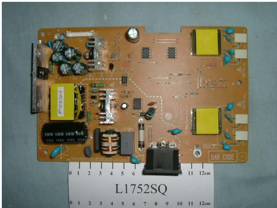
FIGURE 13 LCD MONITOR (M/N: L1752SQ) POWER BOARD (COMPONENT SIDE)
