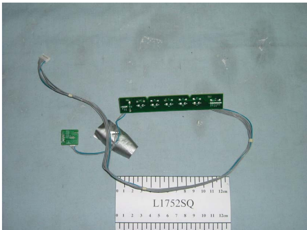
FIGURE 20 LCD MONITOR (M/N: L1752SQ) CONTROL BOARD (SOLDERED SIDE)
