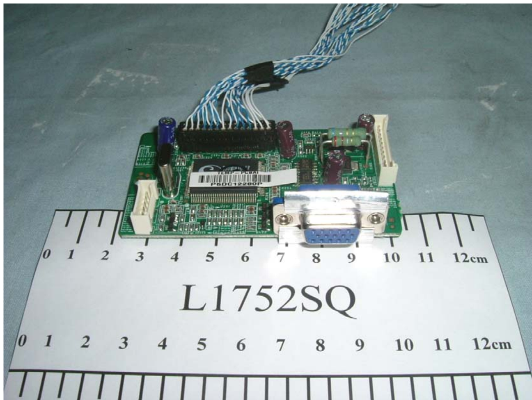
FIGURE 17 LCD MONITOR (M/N: L1752SQ) VGA PORT
