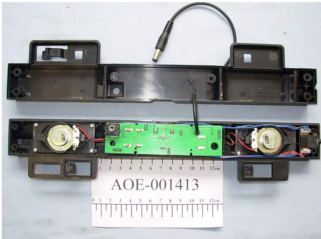
FIGURE 22 LCD MONITOR (M/N: L1753HMS) SPEAKER COVER REMOVED
