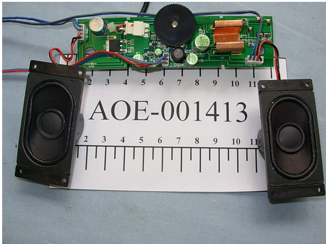
FIGURE 23 LCD MONITOR (M/N: L1753HMS) SPEAKER MAIN BOARD & TRUMPET FRONT
