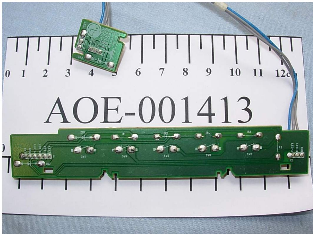
FIGURE 4 LCD MONITOR (M/N: L1753HMS) BOARDS REMOVED
