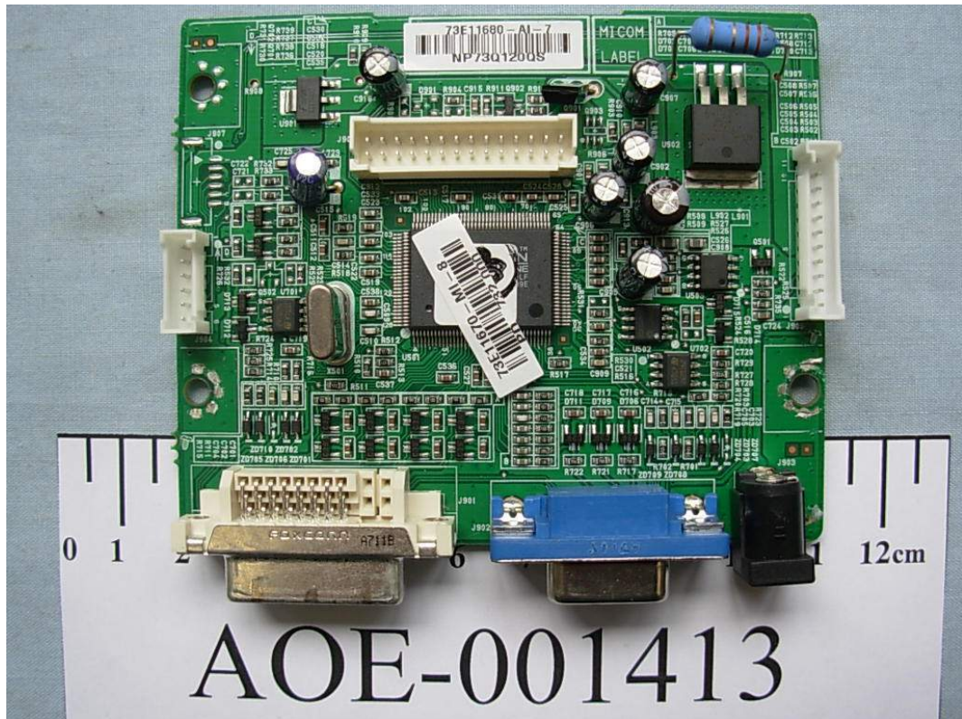
FIGURE 6 LCD MONITOR (M/N: L1753HMS) MAIN BOARD (SOLDERED SIDE)
