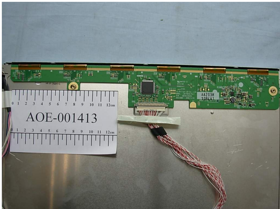
FIGURE 15 LCD MONITOR (M/N: L1753HMS) LCD PANEL MAIN BOARD (SOLDERED SIDE)
