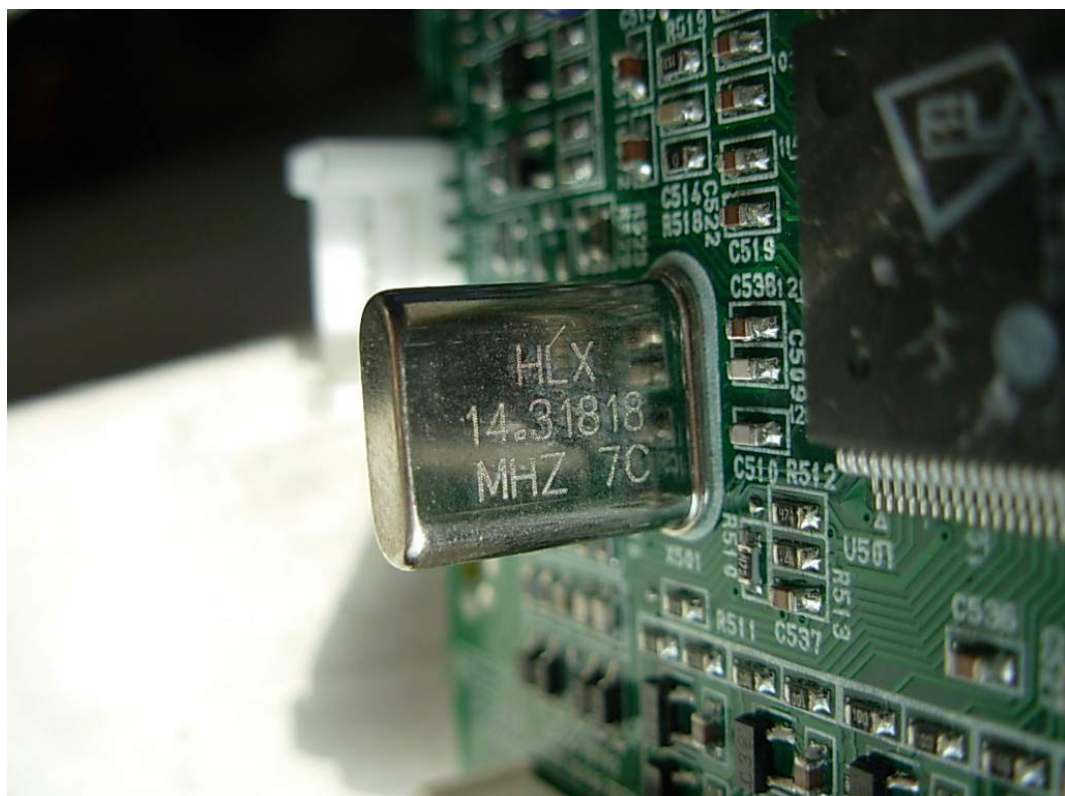
FIGURE 9 LCD MONITOR (M/N: L1753HMS) POWER BOARD (COMPONENT SIDE)
