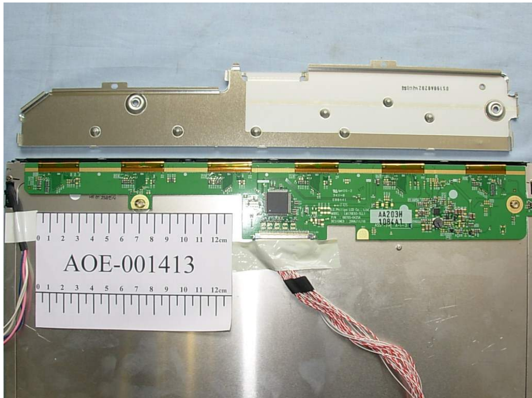
FIGURE 14 LCD MONITOR (M/N: L1753HMS) LCD PANEL MAIN BOARD (COMPONENT SIDE)
