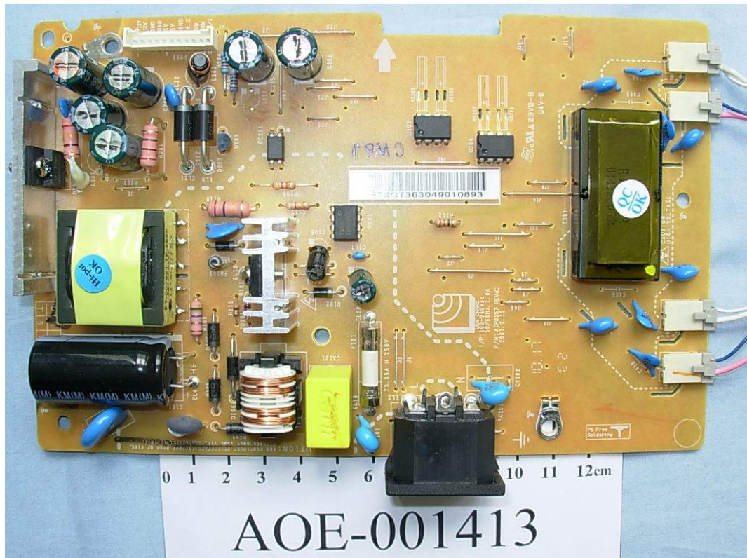
FIGURE 10 LCD MONITOR (M/N: L1753HMS) POWER BOARD (SOLDERED SIDE)
