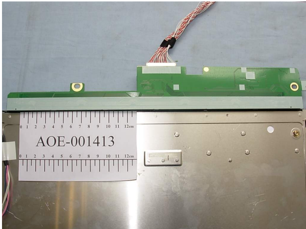
FIGURE 16 LCD MONITOR (M/N: L1753HMS) CHIP ON LCD PANEL MAIN BOARD
