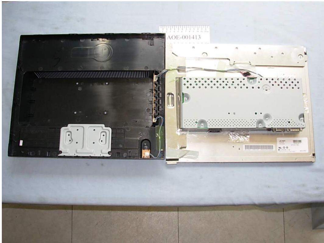
FIGURE 1 LCD MONITOR (M/N: L1753HMS) COVER REMOVED
