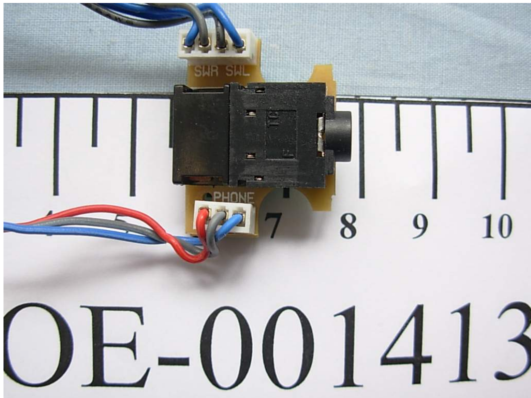
FIGURE 26 LCD MONITOR (M/N: L1753HMS) SPEAKER PORT BOARD BACK
