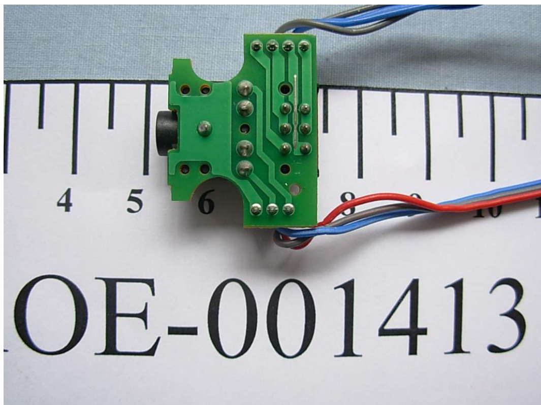
FIGURE 27 LCD MONITOR (M/N: L1753HMS) DEBUG 1
