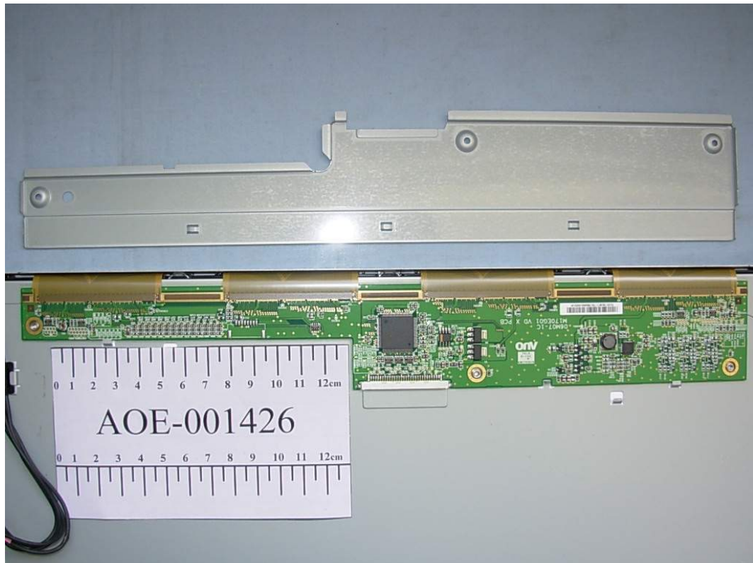
FIGURE 16 LCD MONITOR (M/N: L1754SMS) LCD PANEL MAIN BOARD FRONT
