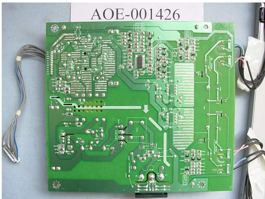
FIGURE 12 LCD MONITOR (M/N: L1754SMS) POWER BOARD (SOLDERED SIDE)
