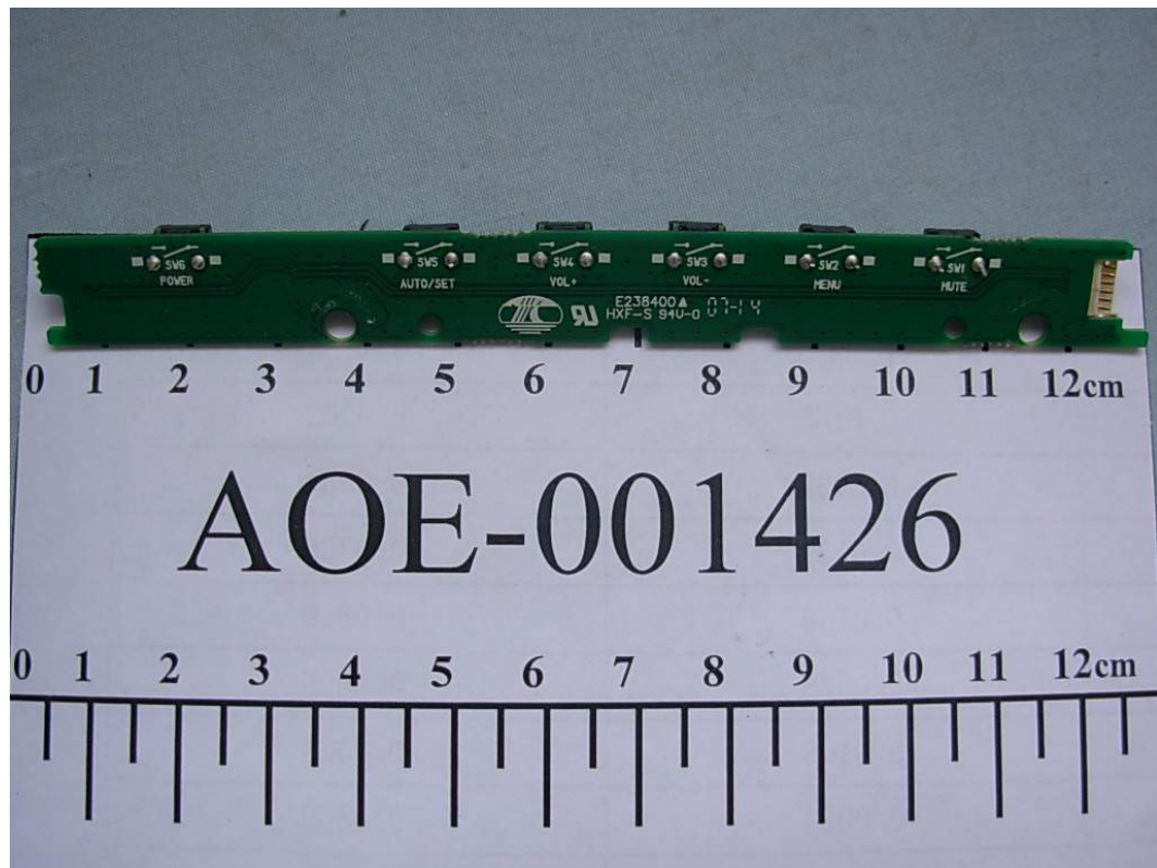
FIGURE 6 LCD MONITOR (M/N: L1754SMS) BOARDS REMOVED
