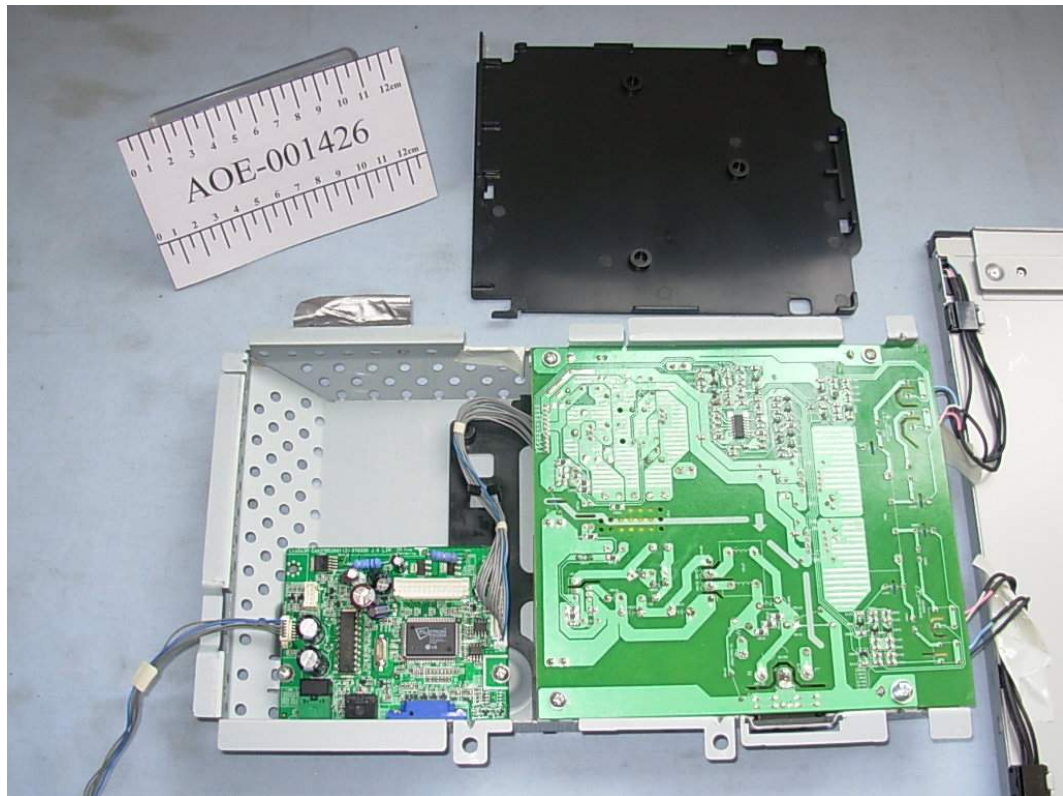
FIGURE 8 LCD MONITOR (M/N: L1754SMS) MAIN BOARD (COMPONENT SIDE)
