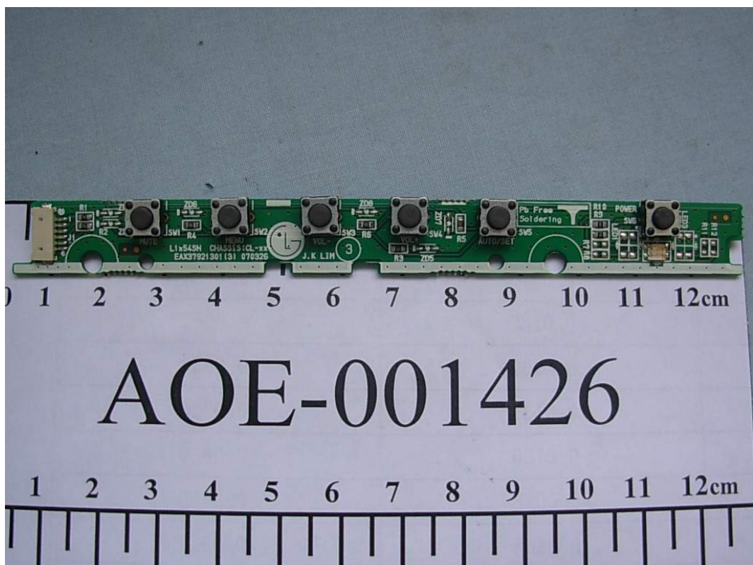
FIGURE 4 LCD MONITOR (M/N: L1754SMS) BUTTON BOARD FRONT
