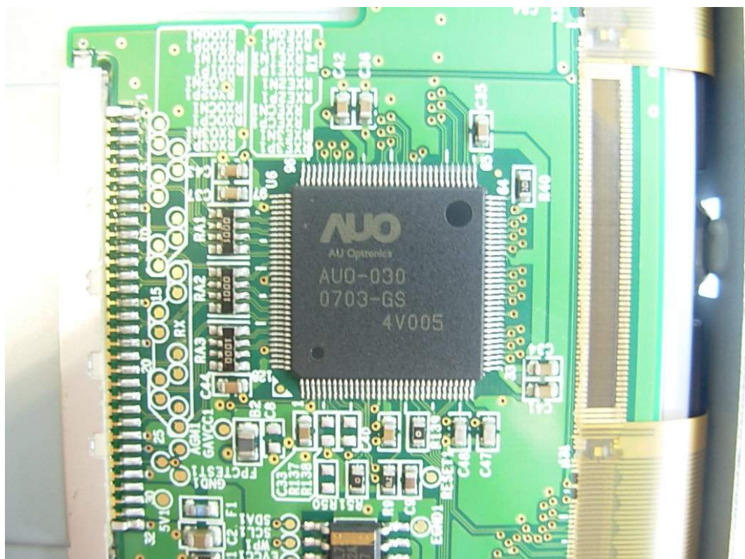
FIGURE 18 LCD MONITOR (M/N: L1754SMS) CHIP ON LCD PANEL MAIN BOARD
