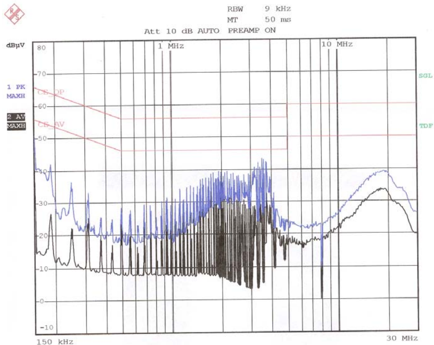
< Neutral line >
