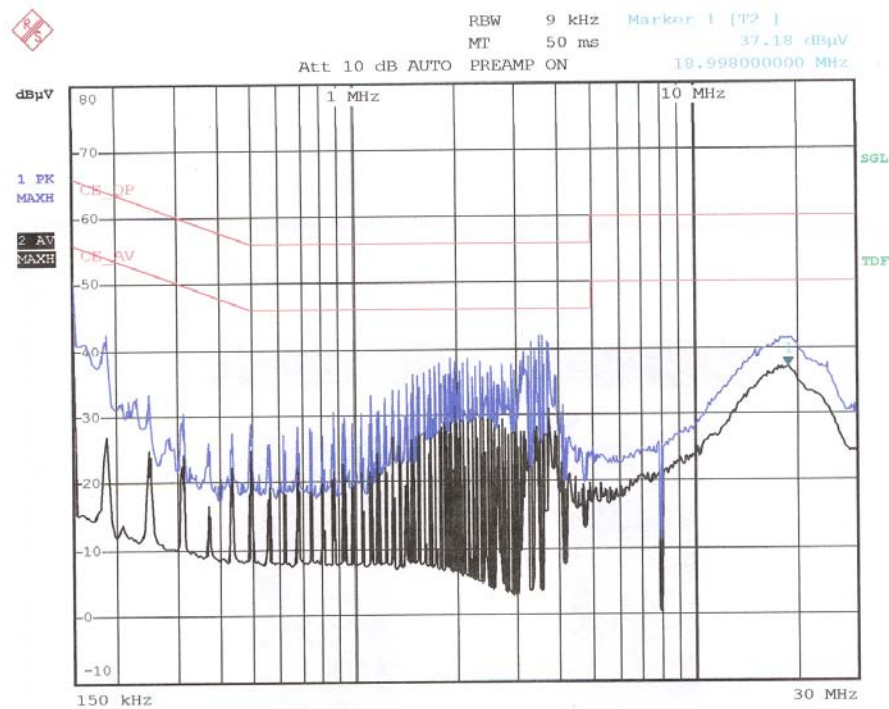
< Hot line >
