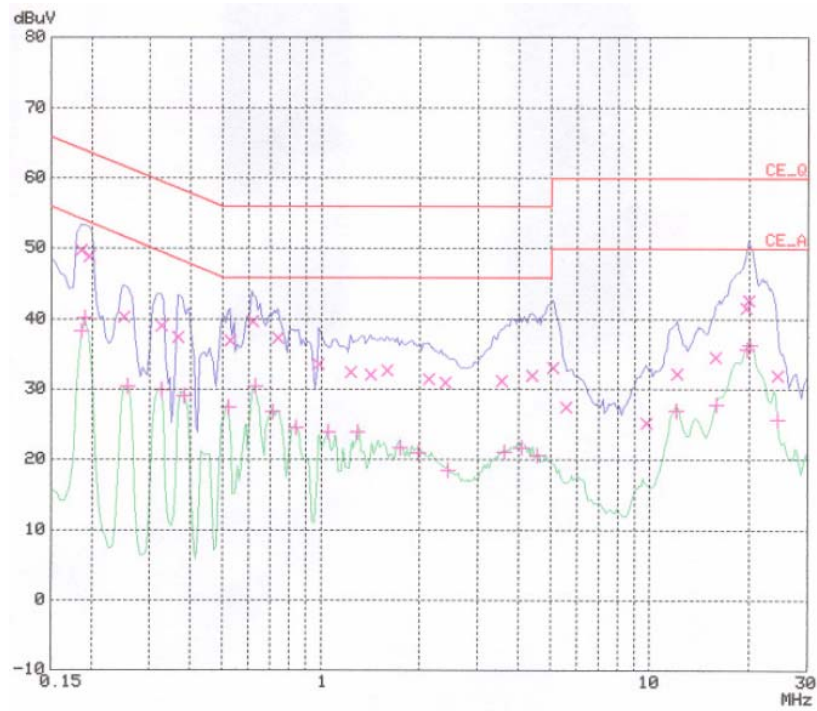
< Hot line >
