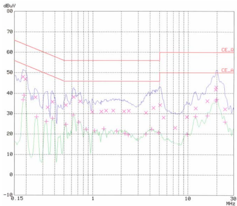
< Neutral line >
