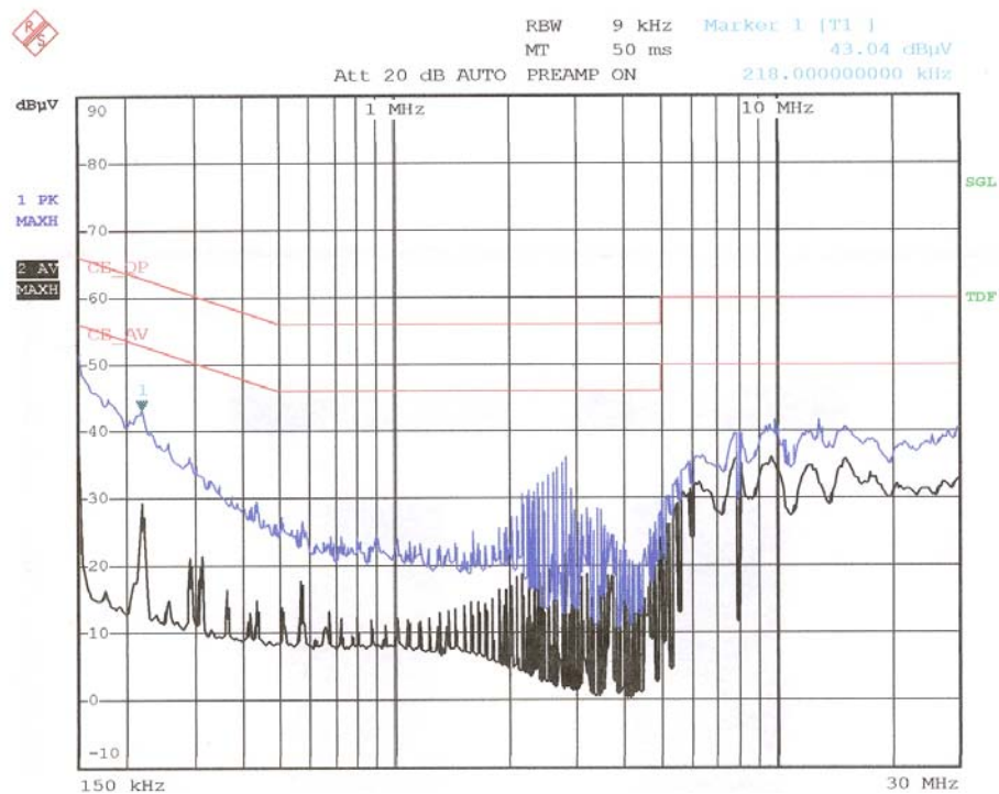
< Hot line >
