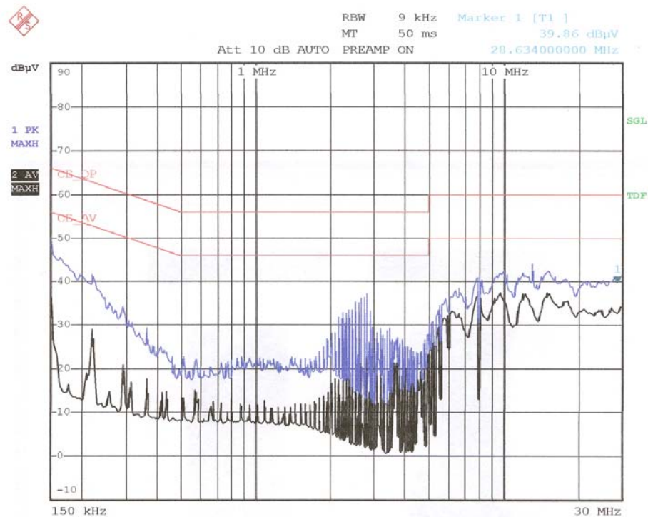
< Neutral line >
