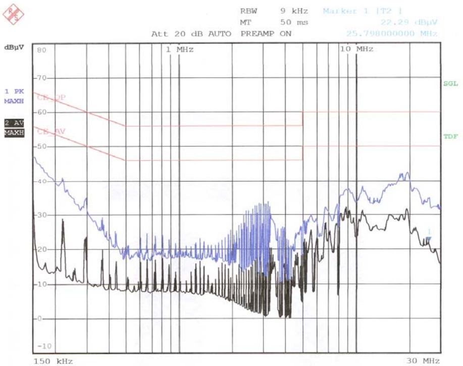
< Neutral line >
