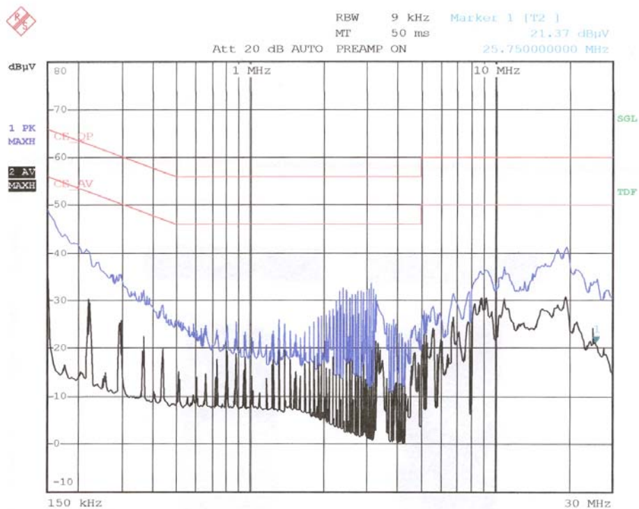
< Hot line >
