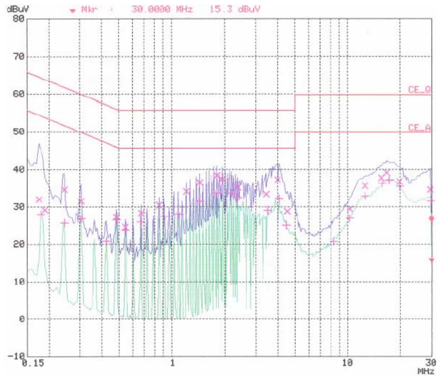
< Neutral line >
