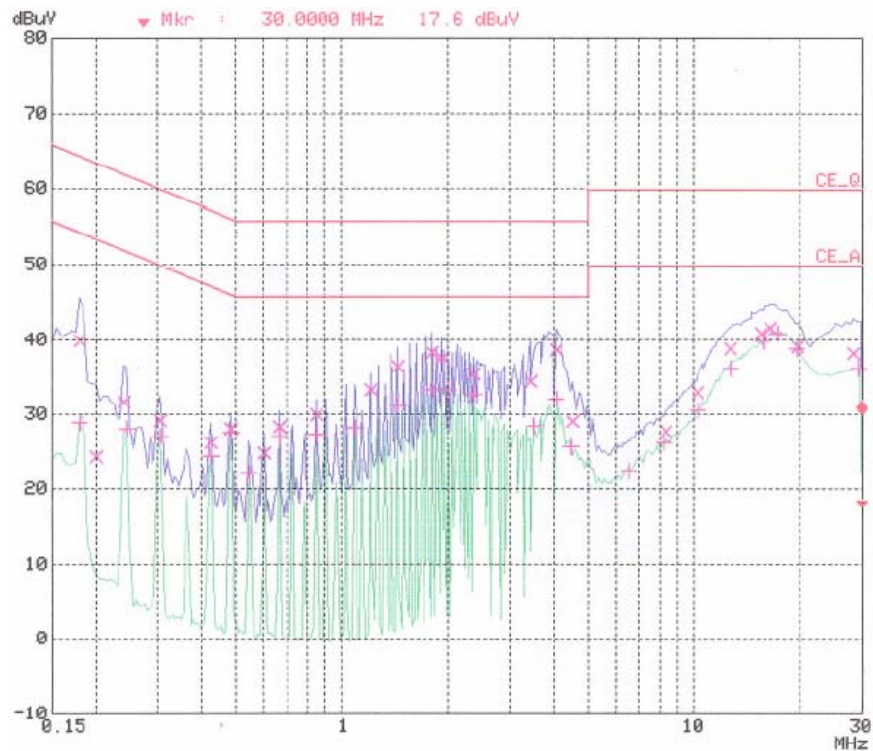
< Hot line >
