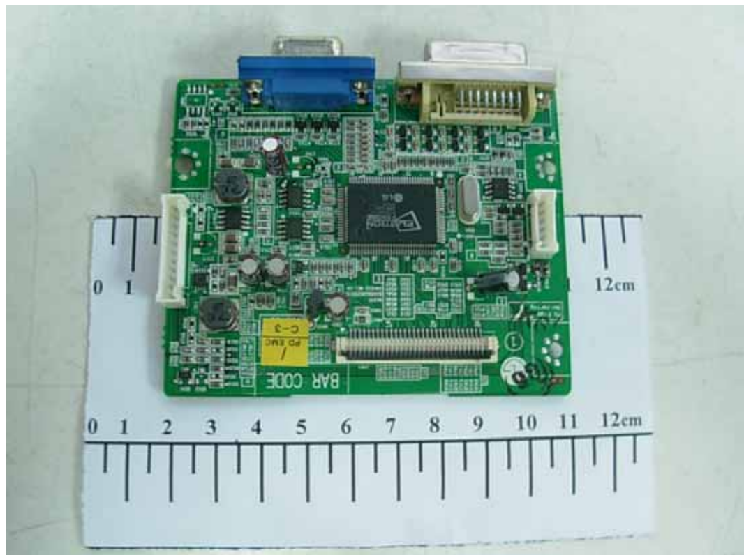
FIGURE 7 LCD MONITOR (M/N: L1942PEU) MAIN BOARD (COMPONENT SIDE)
