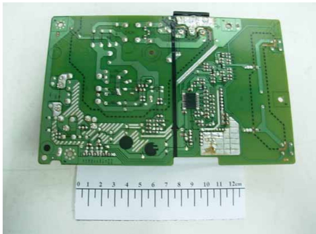
FIGURE 6 LCD MONITOR (M/N: L1942PEU) POWER BOARD (SOLDERED SIDE)
