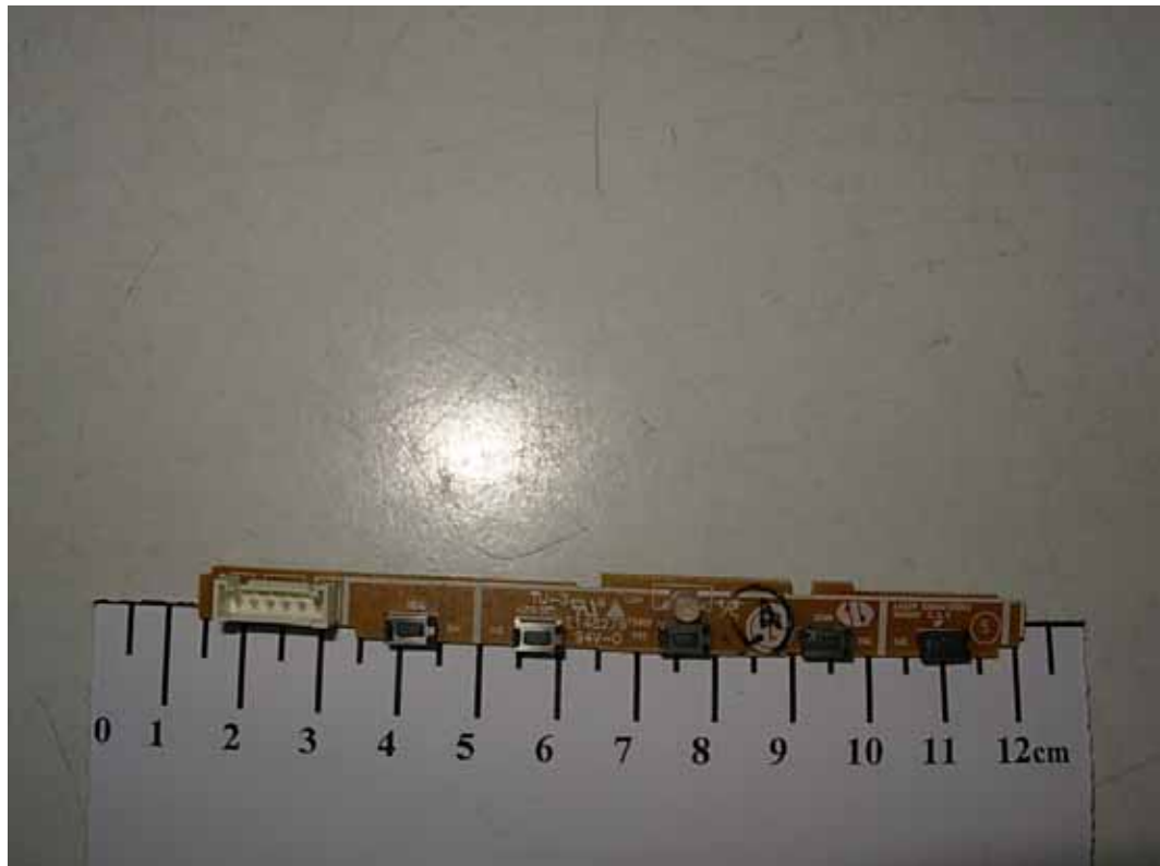
FIGURE 2 LCD MONITOR (M/N: L1942PEU) KEY BOARD (COMPONENT SIDE)
