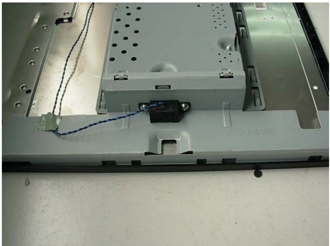
FIGURE 3 LCD MONITOR (M/N: L1942SMT) SPEAKER #2
