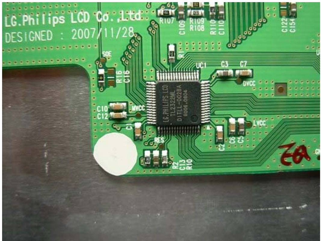
FIGURE 17 LCD MONITOR (M/N: L1942SMT) CHIP ON LCD PANEL MAIN BOARD
