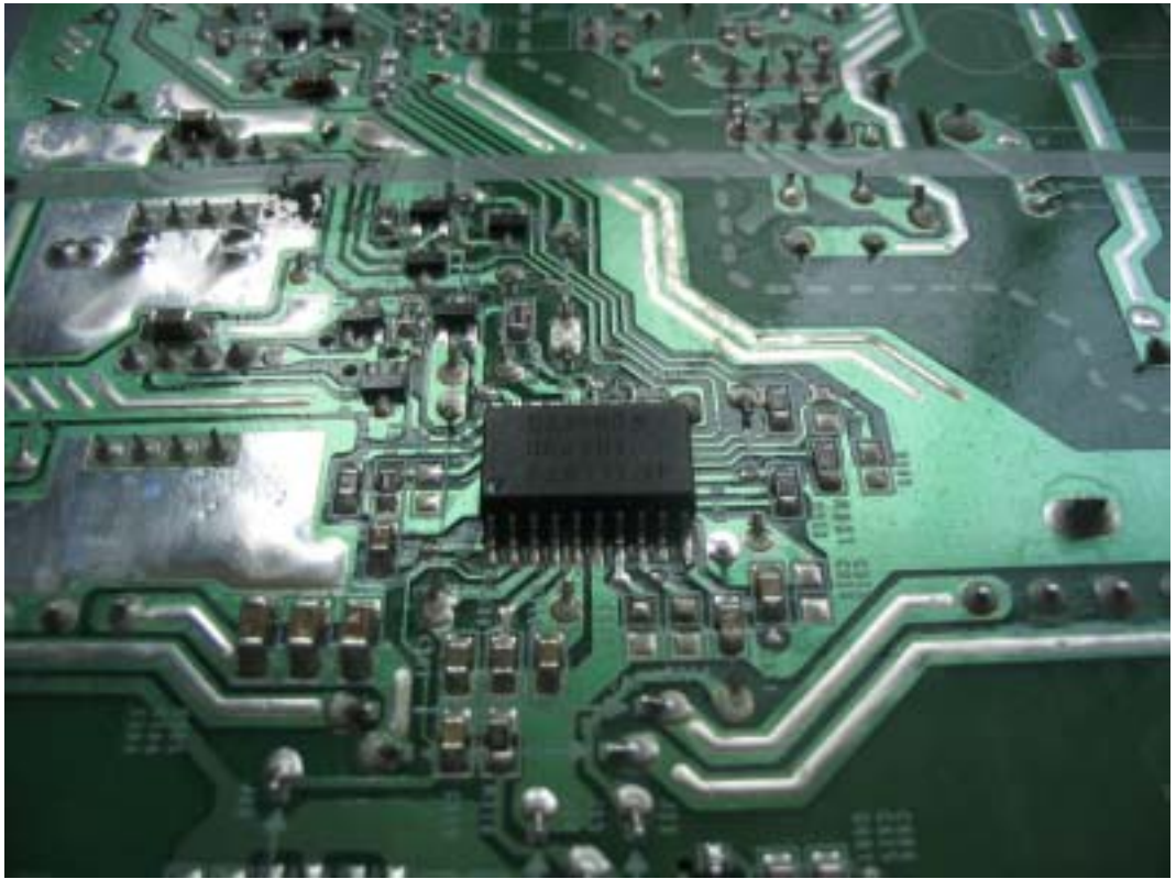
FIGURE 13 LCD MONITOR (M/N: L194WTM) POWER SUPPLY BOARD - IC
