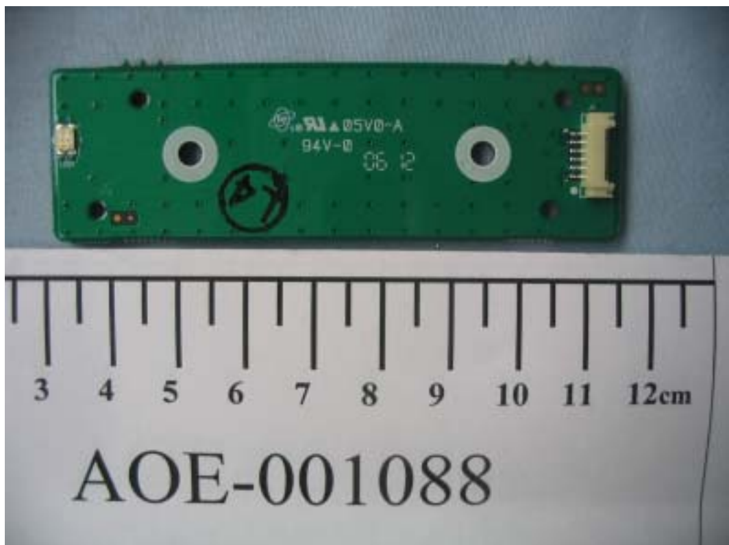
FIGURE 6 LCD MONITOR (M/N: L194WTM) CONTROL BOARD (SOLDERED SIDE)
