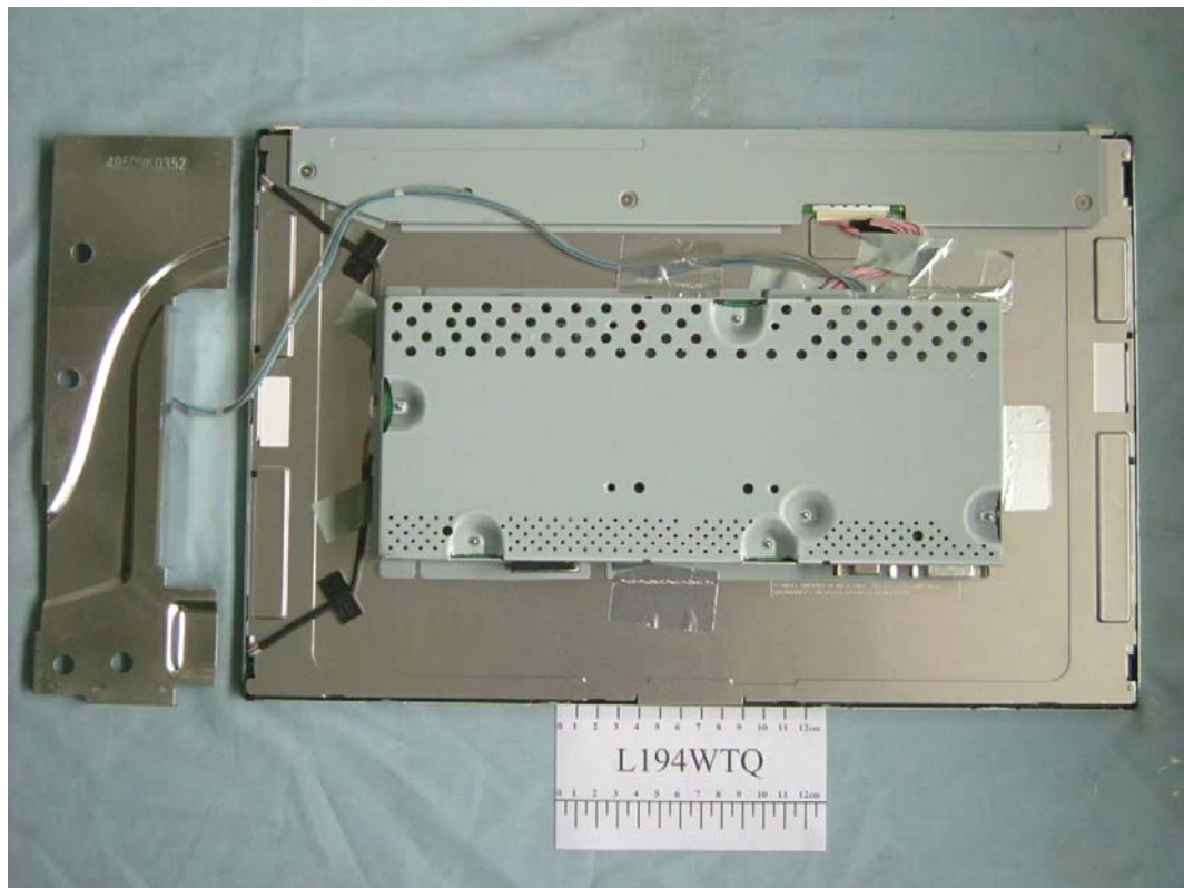
FIGURE 2 LCD MONITOR (M/N: L194WTQ) SHIELDED SHELL 1 REMOVED
