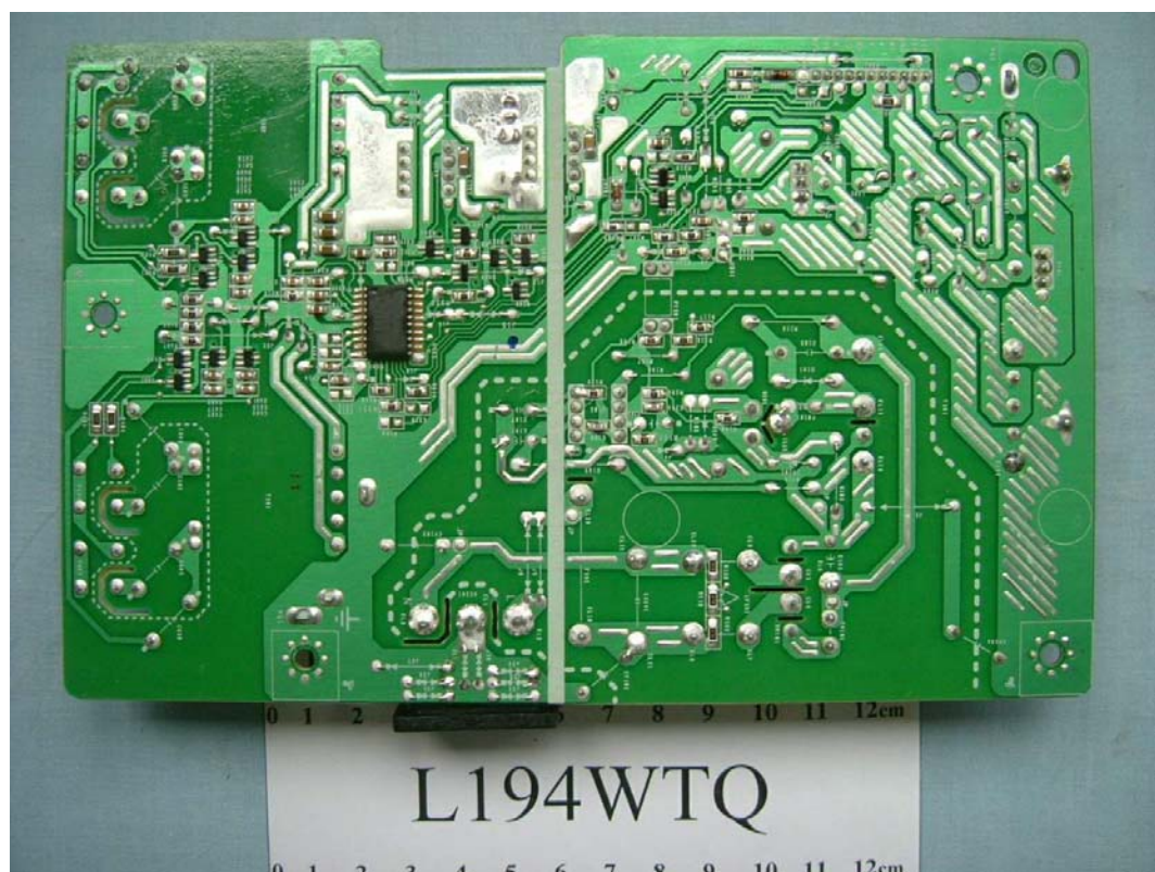
FIGURE 10 LCD MONITOR (M/N: L194WTQ) POWER BOARD (SOLDERED SIDE)
