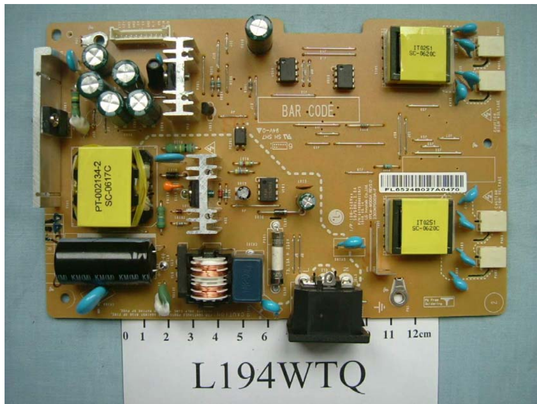
FIGURE 9 LCD MONITOR (M/N: L194WTQ) POWER BOARD (COMPONENT SIDE)
