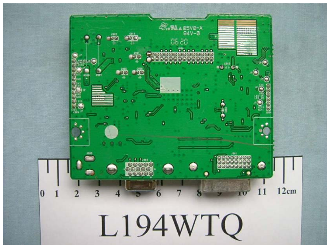
FIGURE 6 LCD MONITOR (M/N: L194WTQ) MAIN BOARD (SOLDERED SIDE)
