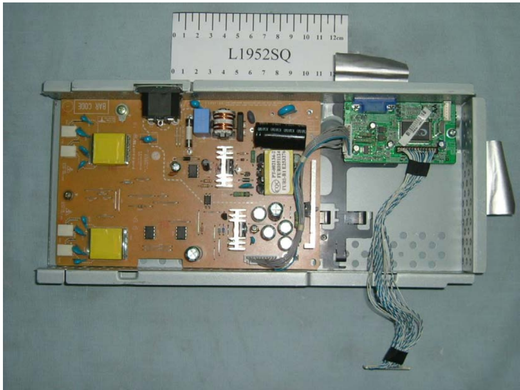
FIGURE 11 LCD MONITOR (M/N: L1952SQ) SHIELDED CASE INSIDE 1
