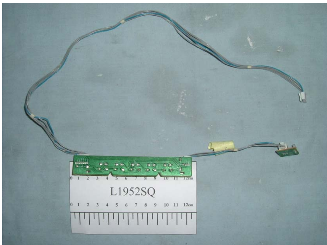
FIGURE 18 LCD MONITOR (M/N: L1952SQ) CONTROL BOARD (SOLDERED SIDE)
