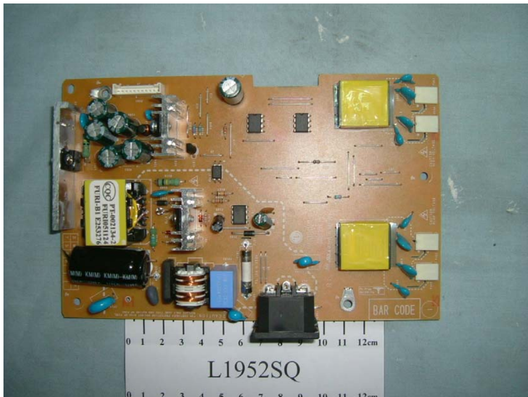
FIGURE 13 LCD MONITOR (M/N: L1952SQ) POWER BOARD (COMPONENT SIDE)
