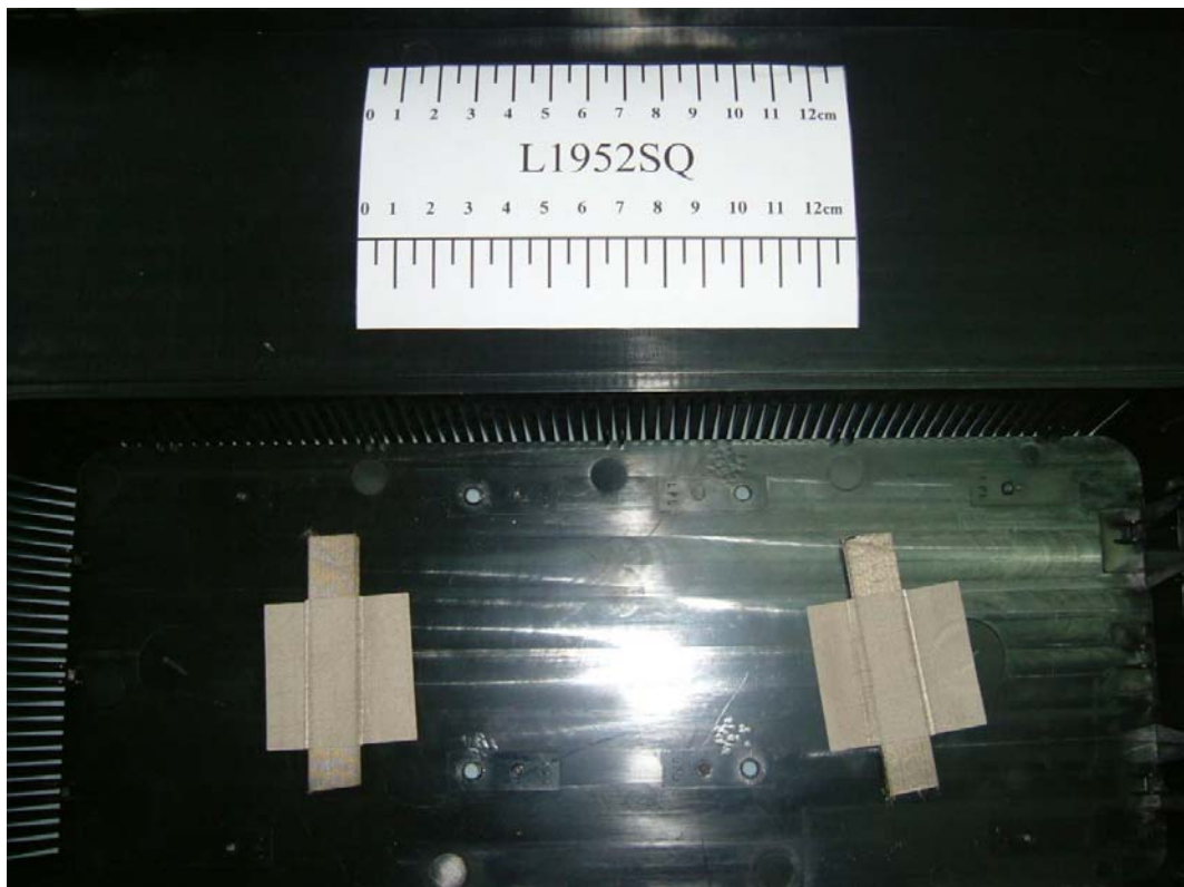
FIGURE 6 LCD MONITOR (M/N: L1952SQ) GASKET IN BACK SHELL
