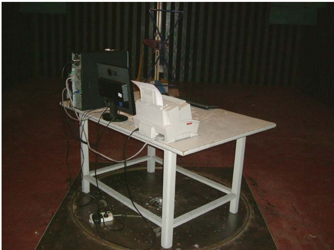
SETUP WITH MAXIMUM DETECTED EMISSION AT VERTICAL POLARIZATION (1280*1024@60Hz)
