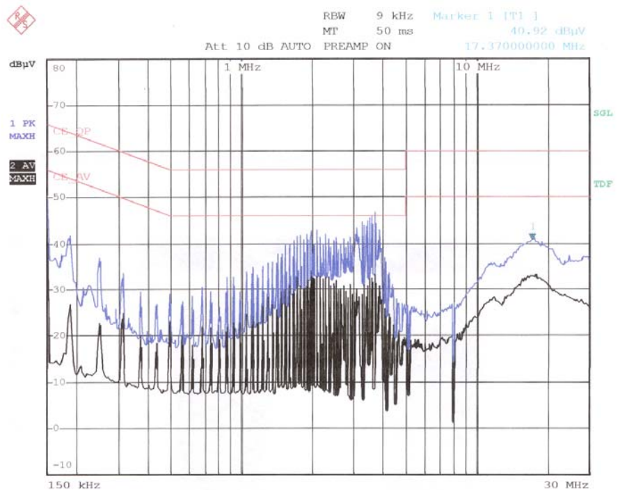
< Neutral line >
