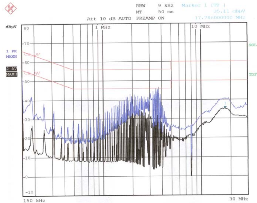
< Neutral line >
