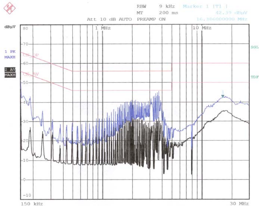
< Hot line >
