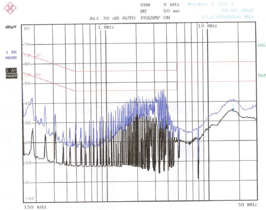
< Neutral line >
