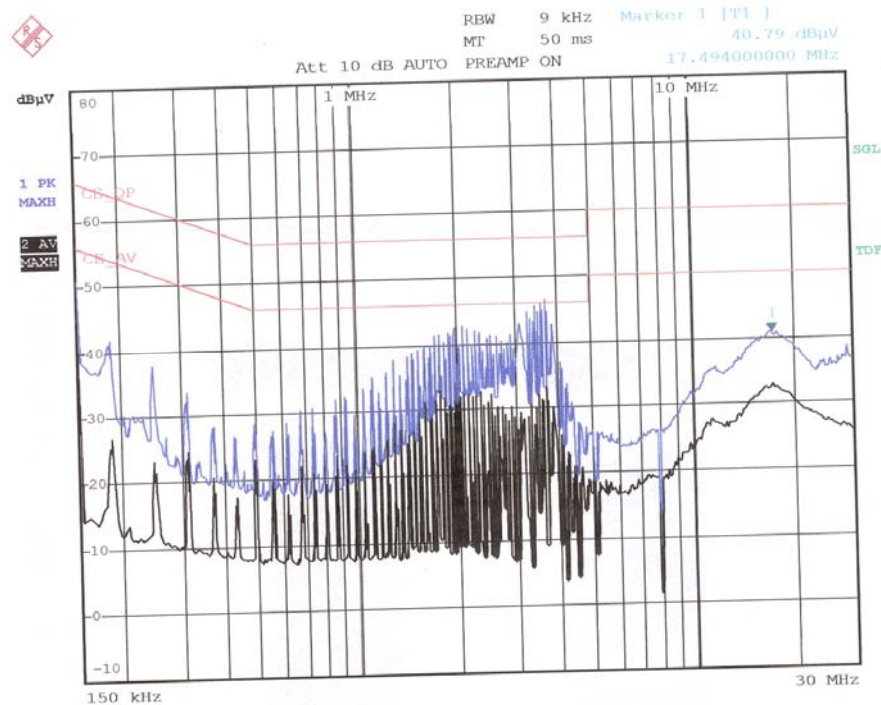
< Neutral line >
