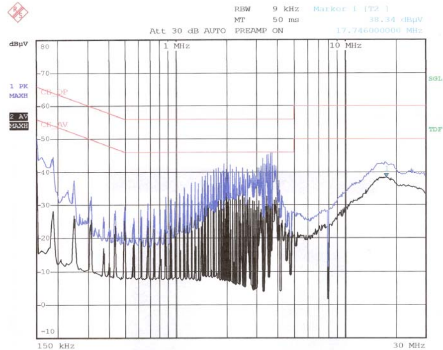
< Hot line >
