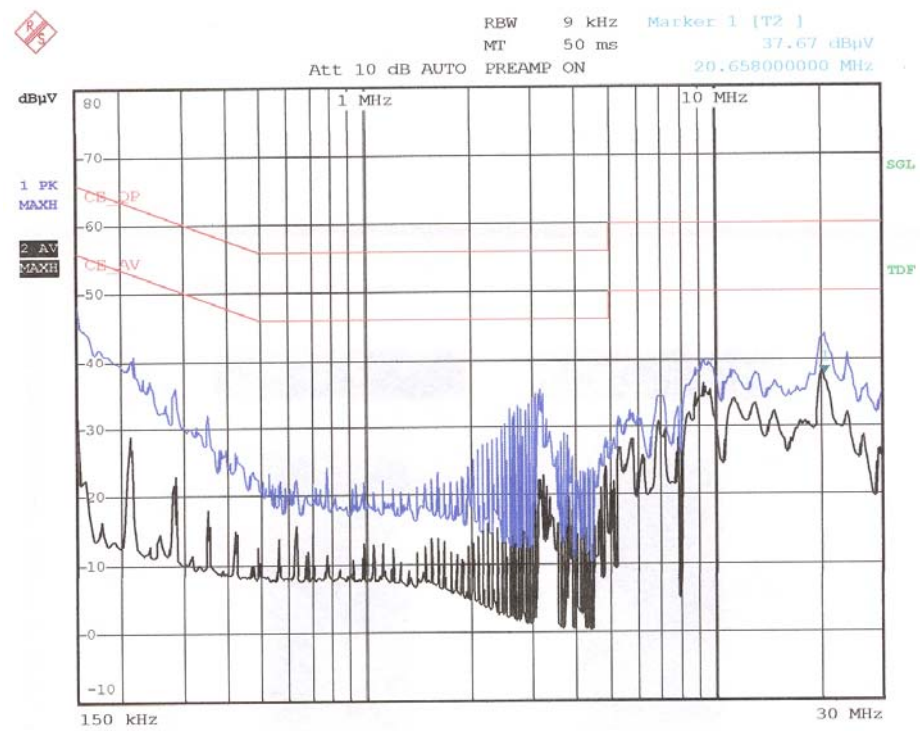
< Neutral line >
