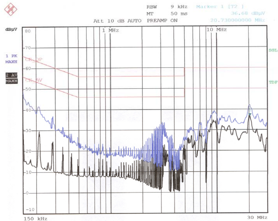
< Hot line >
