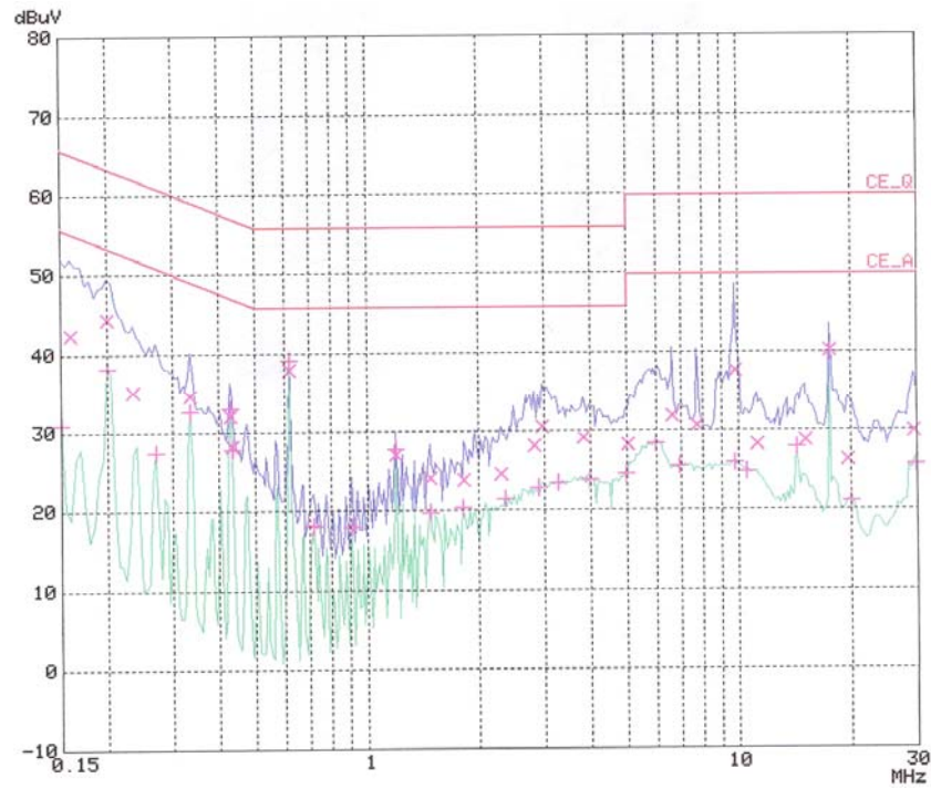
< Hot line >
