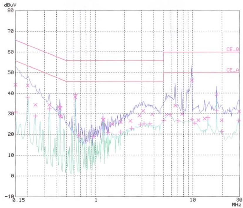
< Hot line >
