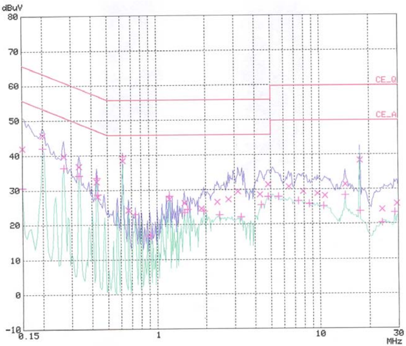
< Neutral line >
