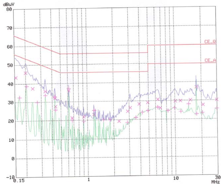
< Neutral line >
