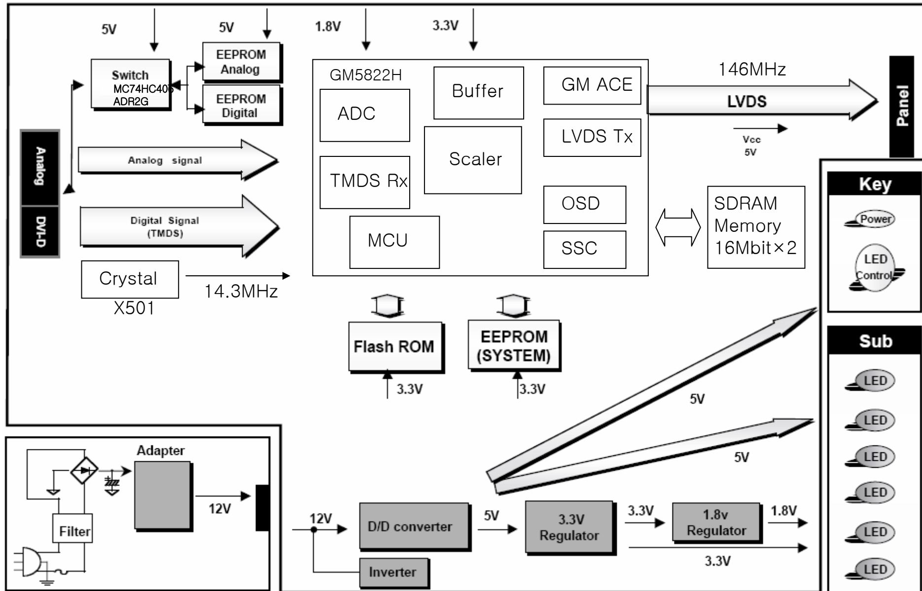
L200WJ-BFQ Block diagram
