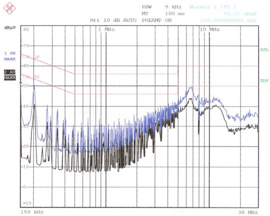
< Hot line >
