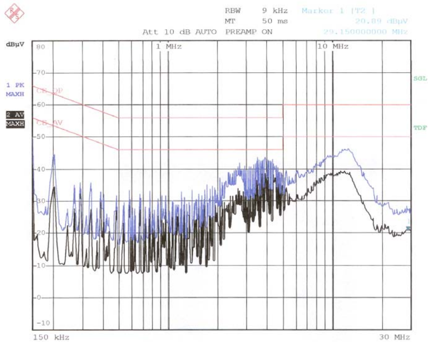
< Hot line >
