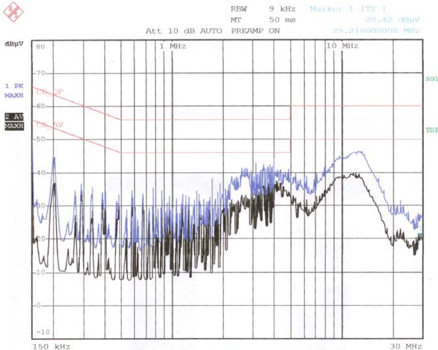
< Neutral line >
