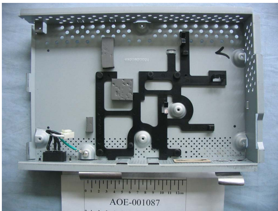
FIGURE 16 LCD MONITOR (M/N: L204WTM) MAIN BOARD – BACK SHELL
