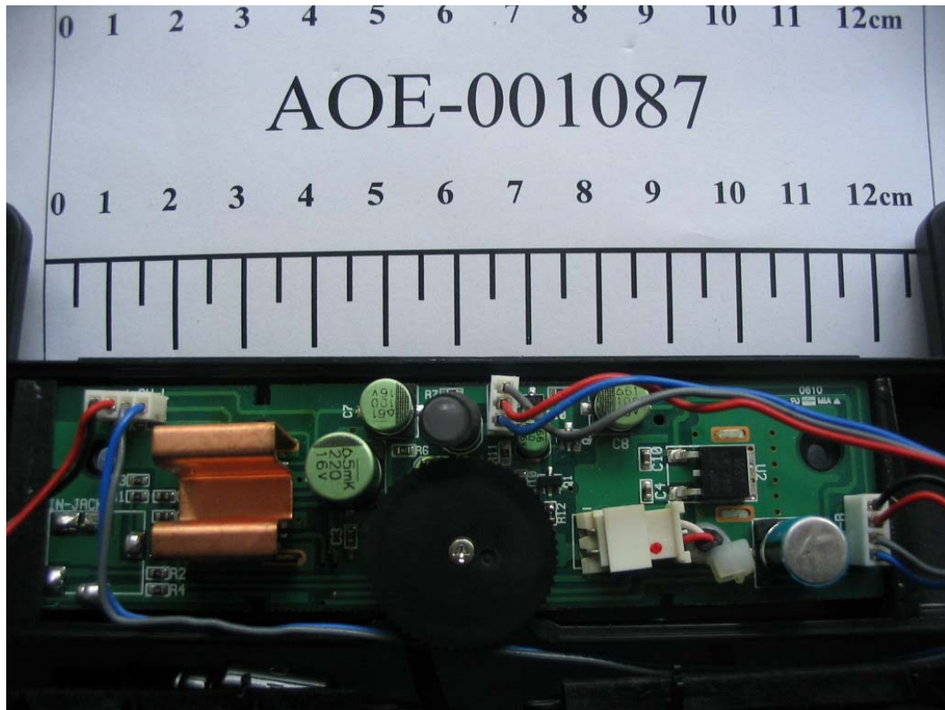
FIGURE 20 LCD MONITOR (M/N: L204WTM) TRUMPET MAIN BOARD (COMPONENT SIDE)
