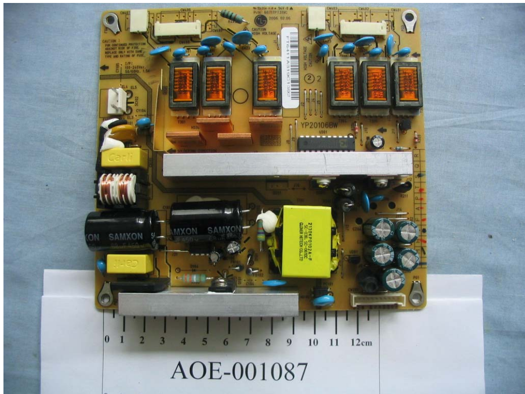
FIGURE 10 LCD MONITOR (M/N: L204WTM) POWER SUPPLY BOARD (COMPONENT SIDE)
