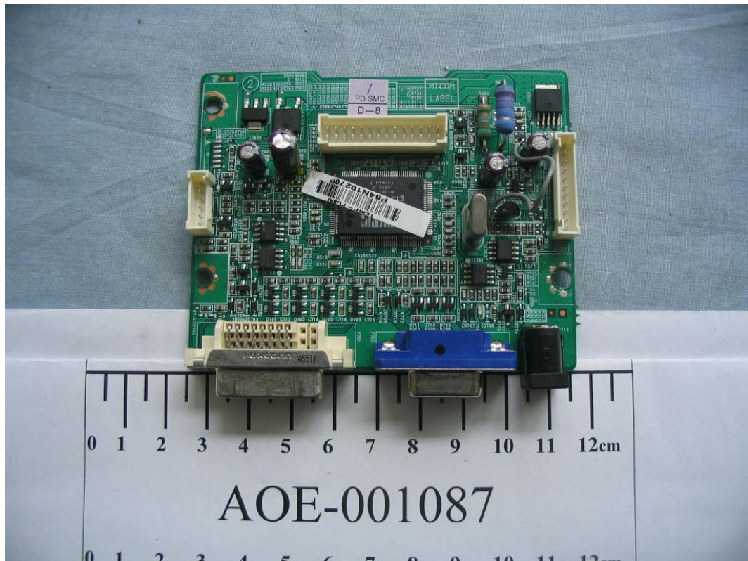
FIGURE 12 LCD MONITOR (M/N: L204WTM) MAIN BOARD (COMPONENT SIDE)
