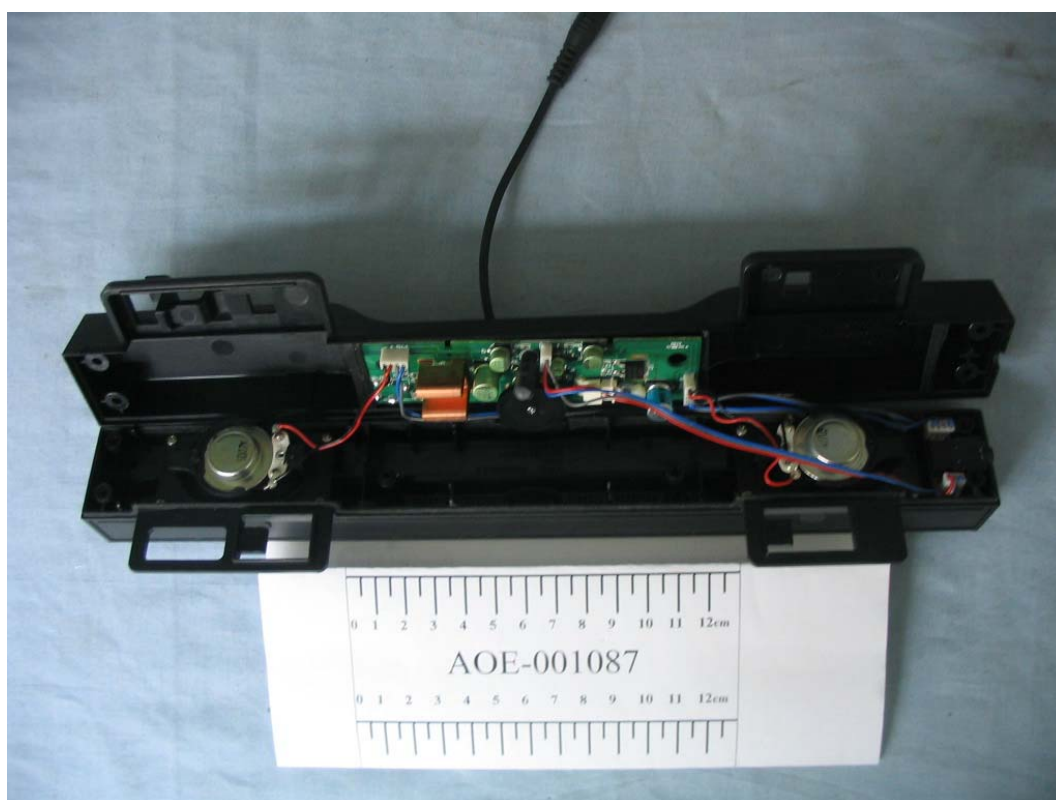
FIGURE 19 LCD MONITOR (M/N: L204WTM) TRUMPET COVER REMOVED
