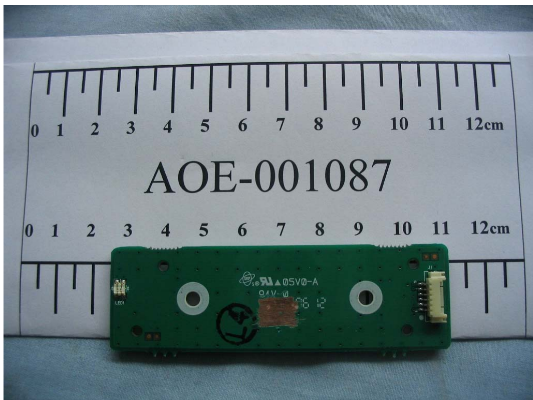
FIGURE 5 LCD MONITOR (M/N: L204WTM) CONTROL BOARD (SOLDERED SIDE)
