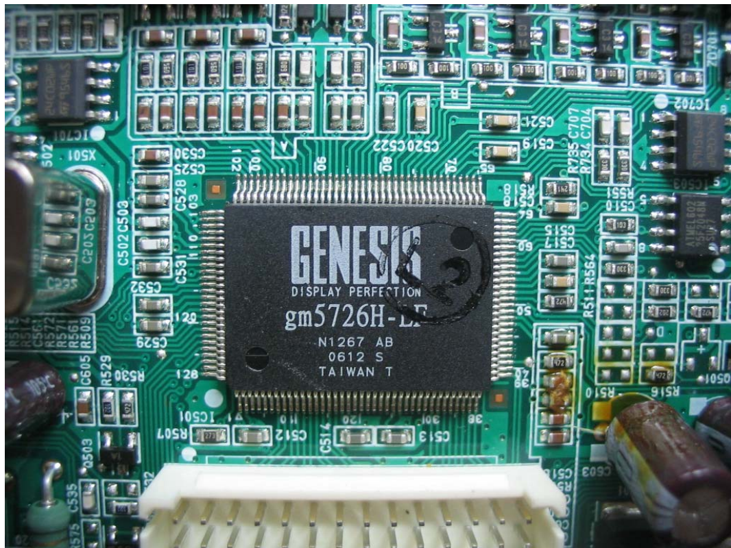
FIGURE 14 LCD MONITOR (M/N: L204WTM) MAIN BOARD - IC
