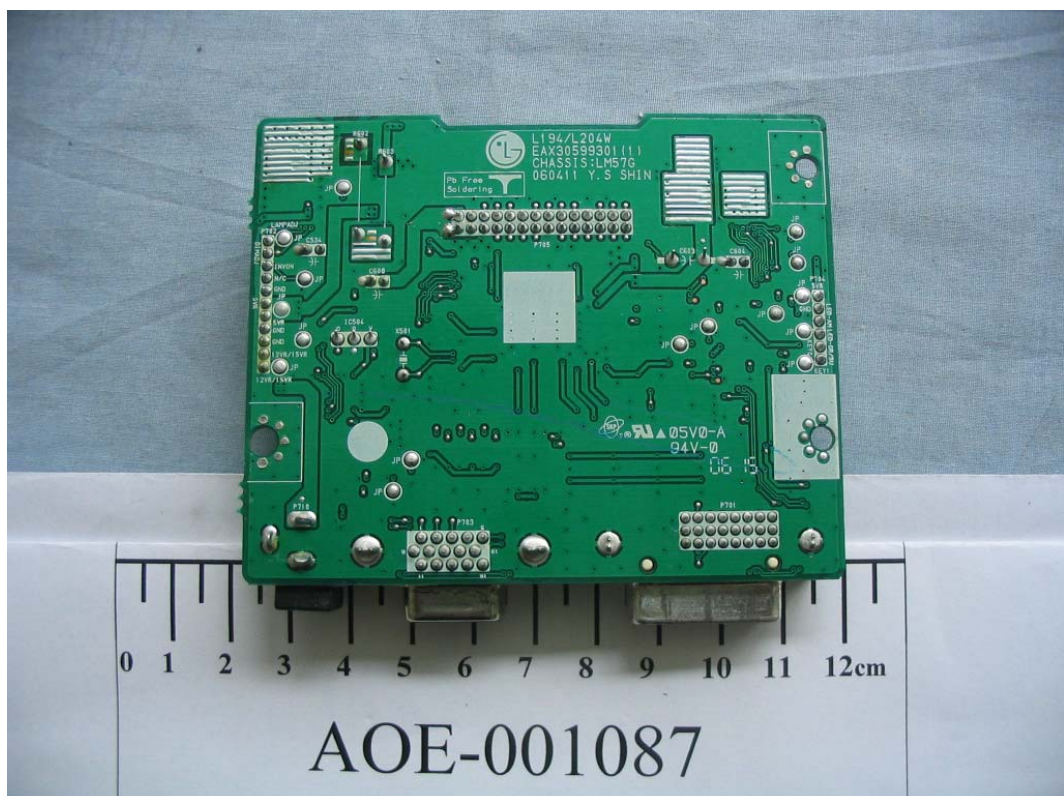
FIGURE 13 LCD MONITOR (M/N: L204WTM) MAIN BOARD (SOLDERED SIDE)
