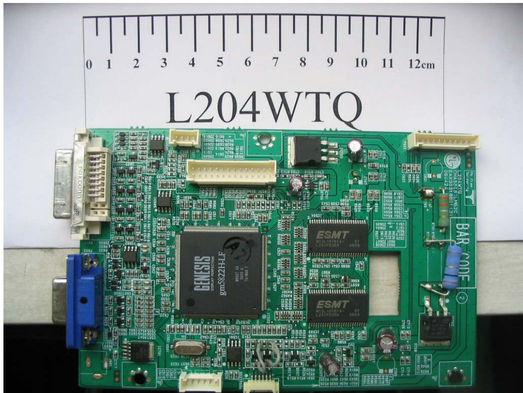
FIGURE 10 LCD MONITOR (M/N: L204WTQ) MAIN BOARD (COMPONENT SIDE)
