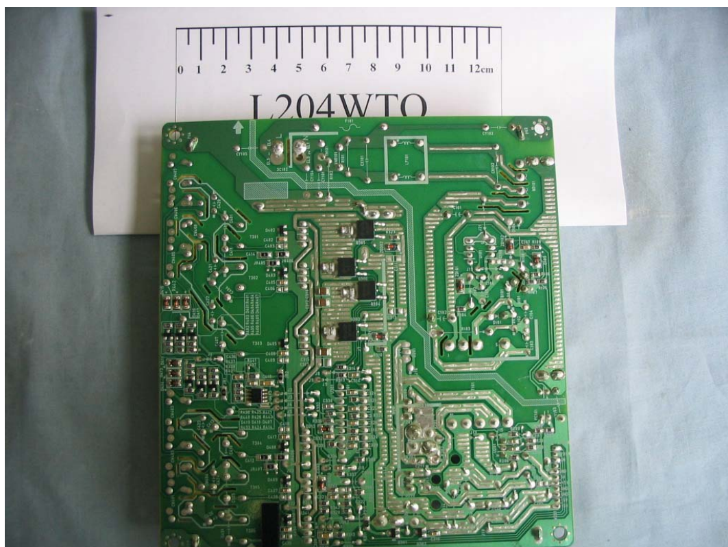
FIGURE 9 LCD MONITOR (M/N: L204WTQ) POWER SUPPLY BOARD (SOLDERED SIDE)
