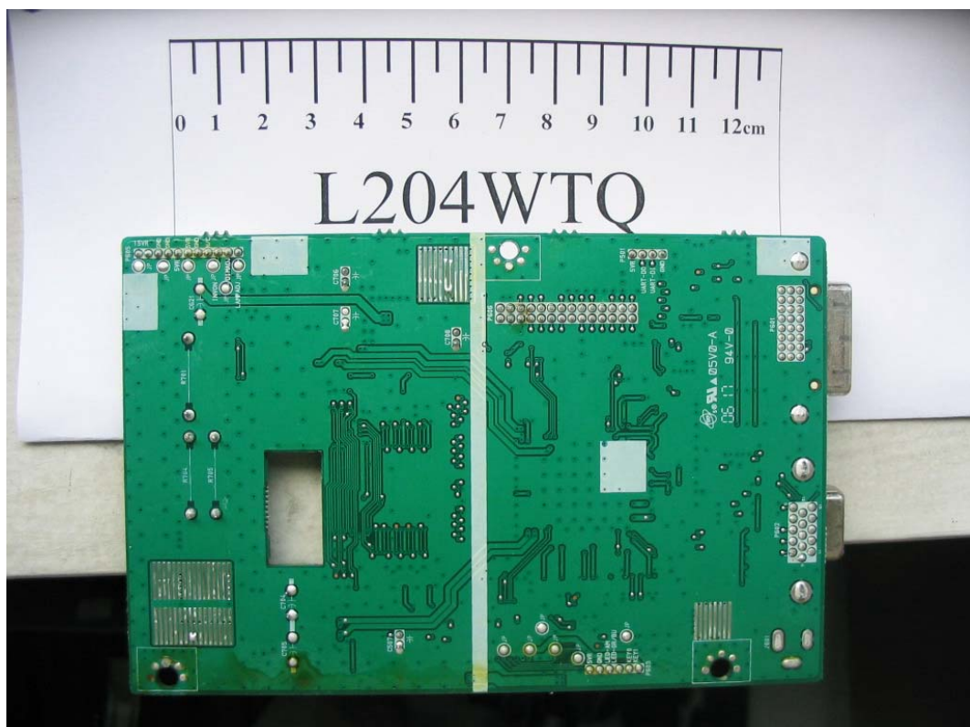
FIGURE 11 LCD MONITOR (M/N: L204WTQ) MAIN BOARD (SOLDERED SIDE)
