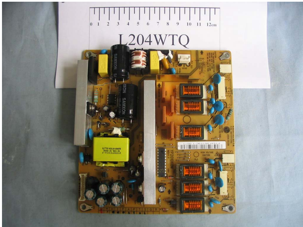
FIGURE 8 LCD MONITOR (M/N: L204WTQ) POWER SUPPLY BOARD (COMPONENT SIDE)
